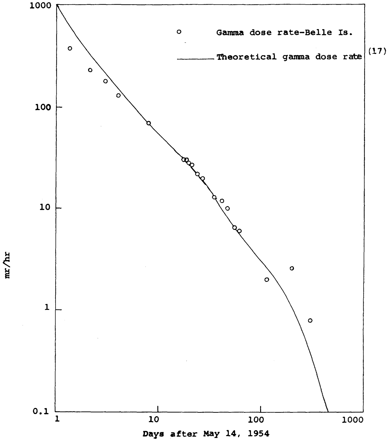
Figure 3. Gamma dose rates at three feet at Belle Island, Eniwetok Atoll, May 15, 1954 to March 21, 1955, compared with the decay of fission products from the slow neutron fission of U^{235} (17).
