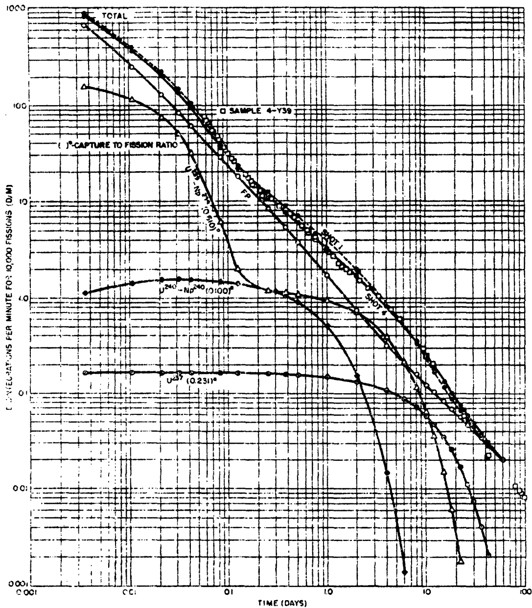
Figure 3.15 Calculated beta decay.
