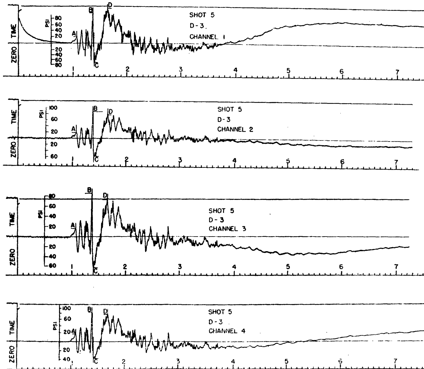
Figure 2.10 Pressure-time records, Shot 5.
