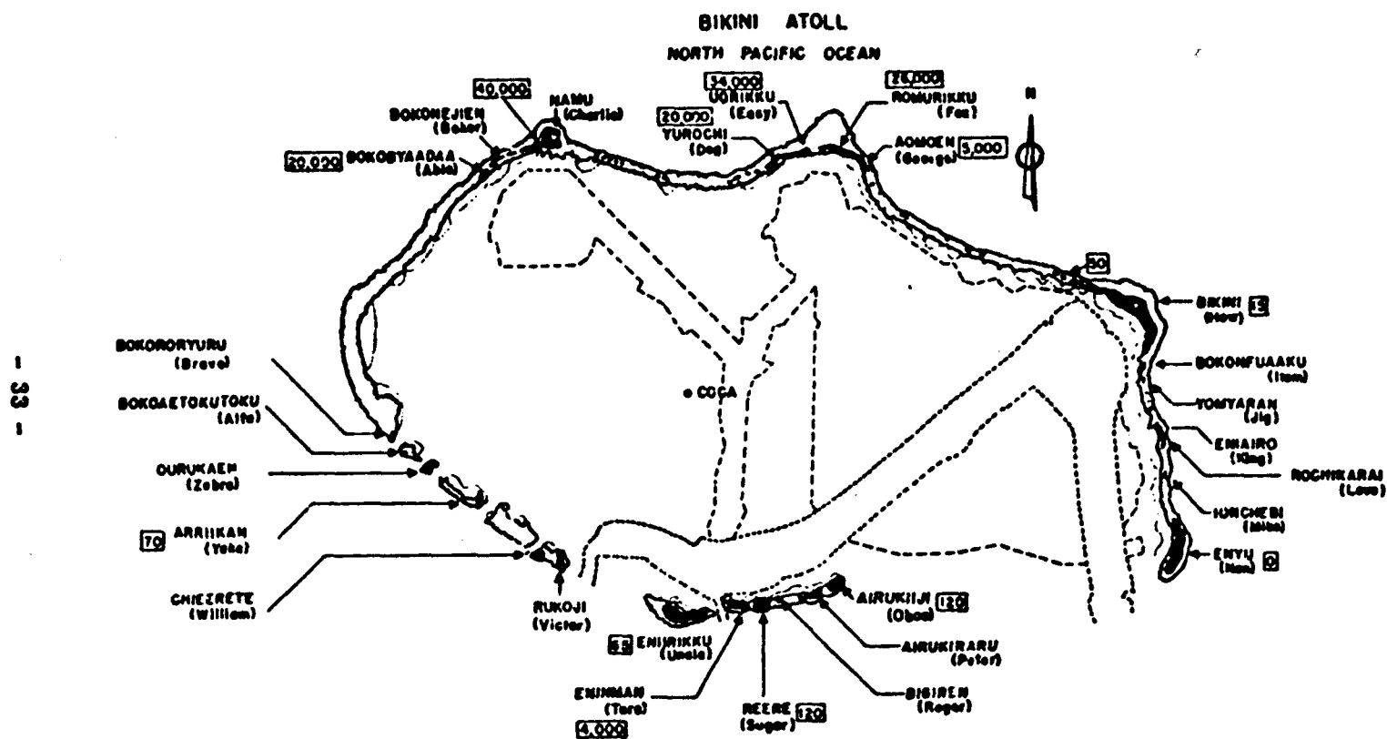
Fig. 3.2 - [Flathead] radiation intensities on Bikini Atoll at H+4 hr, in milliroentgens per hour. Shot site was barge off Yurochi.
