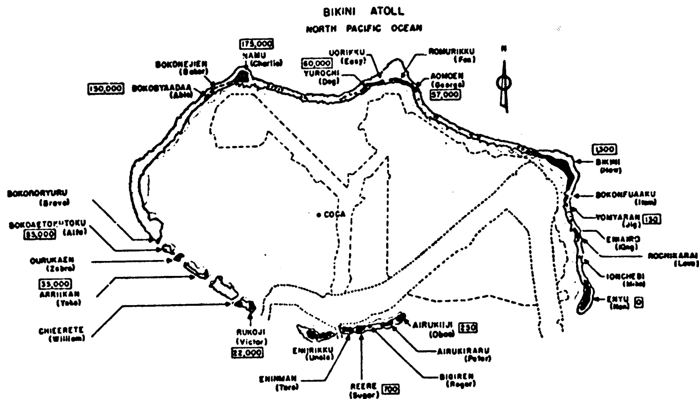
Fig. 3.5- TEWA radiation intensities on Bikini Atoll at H+4 hr, in milliroentgens per hour. Shot site was barge on reef west of Yurochi.
