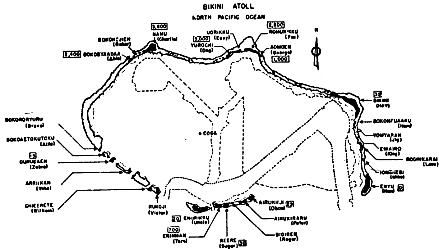
Fig. 3.3 - Dakota radiation intensities on Bikini Atoll at H+4 hr, in milliroentgens per hour. Shot site was barge off Yurochi.
