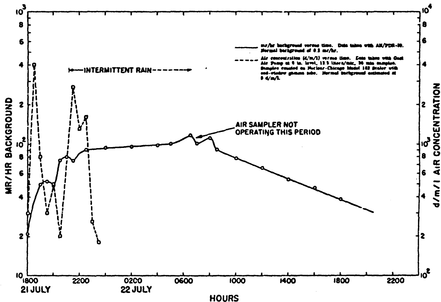
Fig. 2.11—Data on TEWA fall-out at Rad-Safe Building on Parry Island, Eniwetok Atoll, from 1800 hr, 21 July to 2400 hr, 22 July 1956. Shot was fired at Bikini Atoll.
