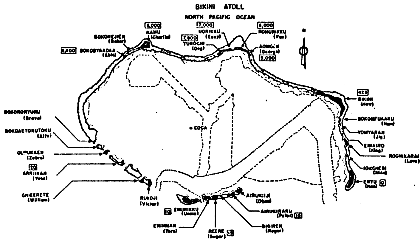
Fig. 3.4 Navajo radiation intensities on Bikini Atoll at H+4 hr, in milliroentgens per hour. Shot site was barge off Yurochi.
