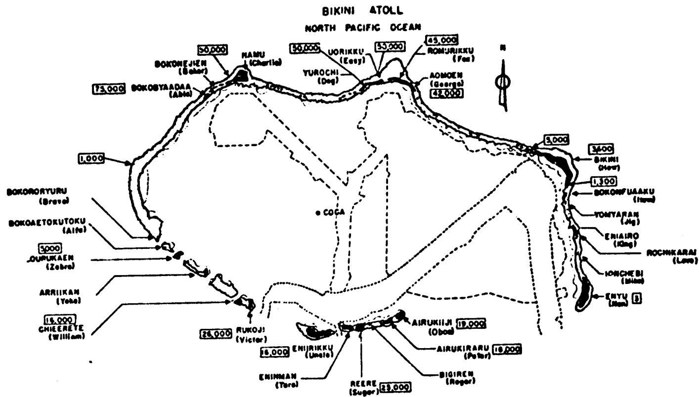
Fig. 3.1 - 137 Zr radiation intensities on Bikini Atoll at H+4 hr, in milliroentgens per hour. Shot island was Eninman.
