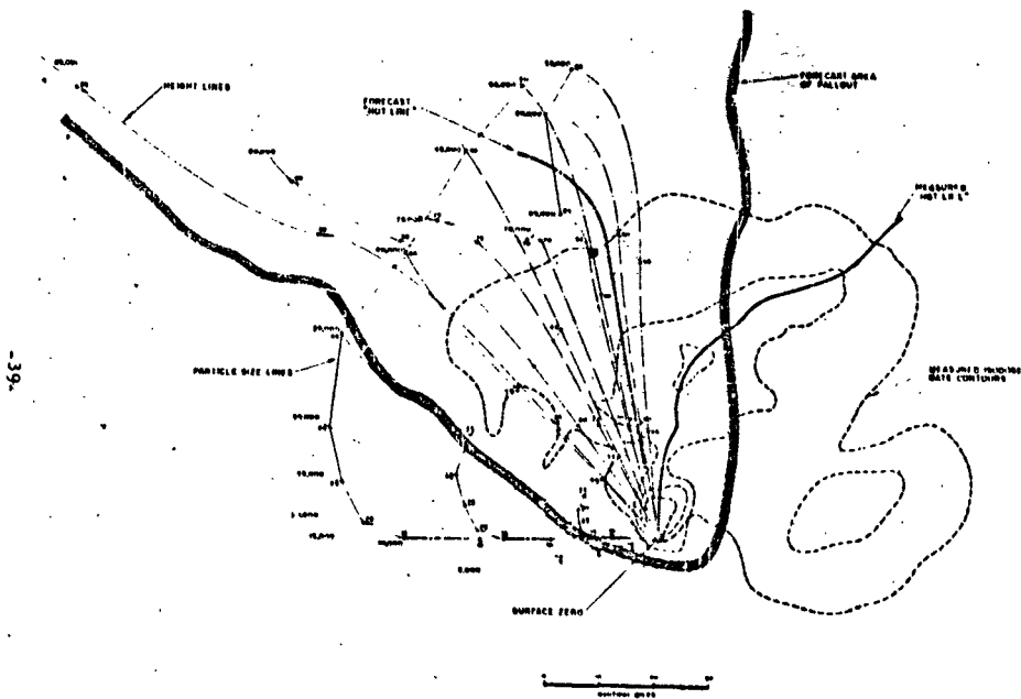
Fig. 13 Comparison of Fallout Forecast With Test Results - Shot B
