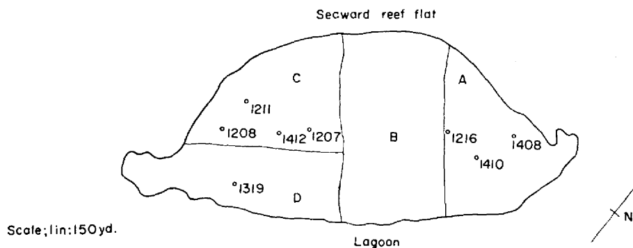
FIG. 2. Diagram of Belle Island, Eniwetok Atoll, showing the location of the land plant stations and the collecting areas.
