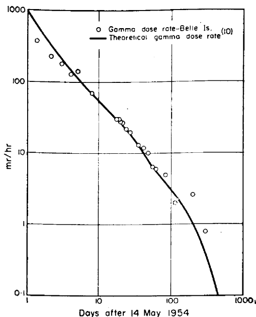
Fig. 3. Gamma dose rates at three feet at Belle Island, Eniwetok Atoll, May 15, 1954 to March 21, 1955, compared with the decay of fission products from the slow neutron fission of U^{235(240)} .
