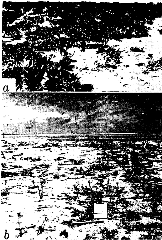
FIG. 4. General view of land plants at Belle Island, Eniwetok Atoll. (a) On April 15, 1954, before the Nectar detonation. (b) On May 22, 1954, eight days following Nectar, showing a Scaevola plant (No. 1319) in the foreground.
