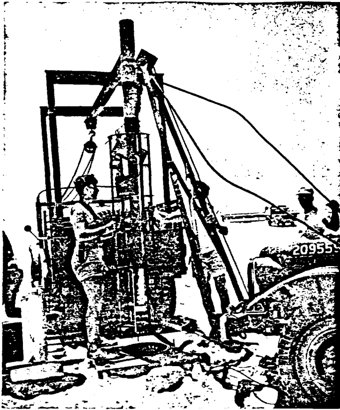
Figure 7 Installation of Emmett device.
