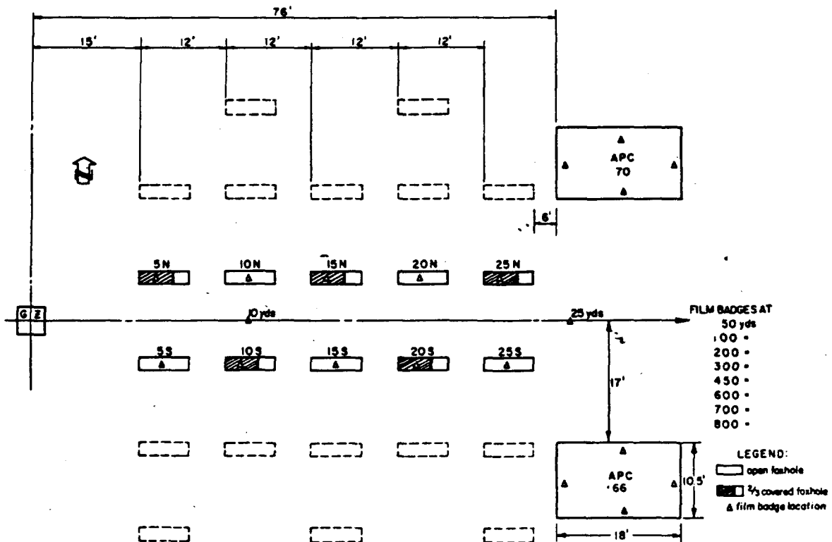
Figure 4 Station layout, Shot Humboldt.
