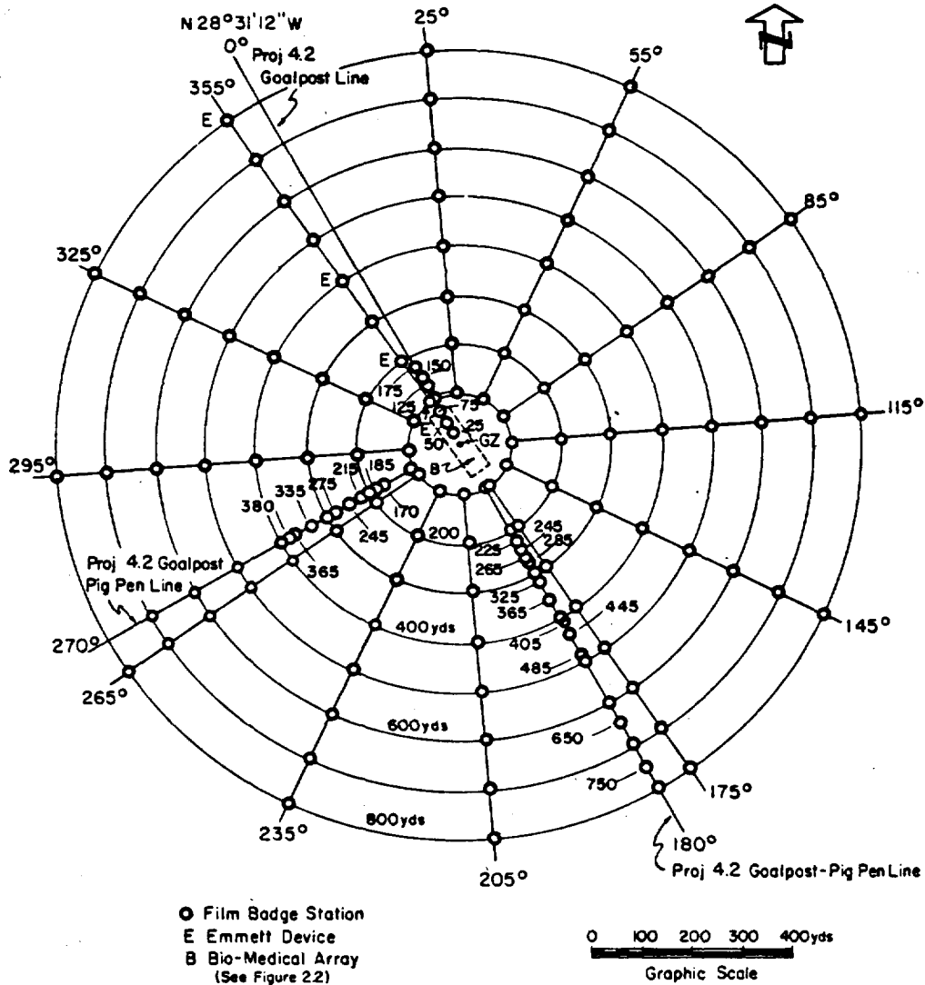
Figure 2 Station layout, Shot Hamilton.
