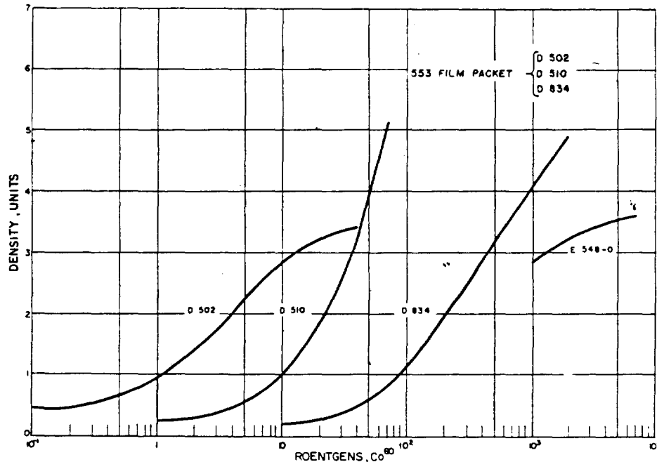
Figure 2.12 Calibration curves for NBS dosimeter film.
