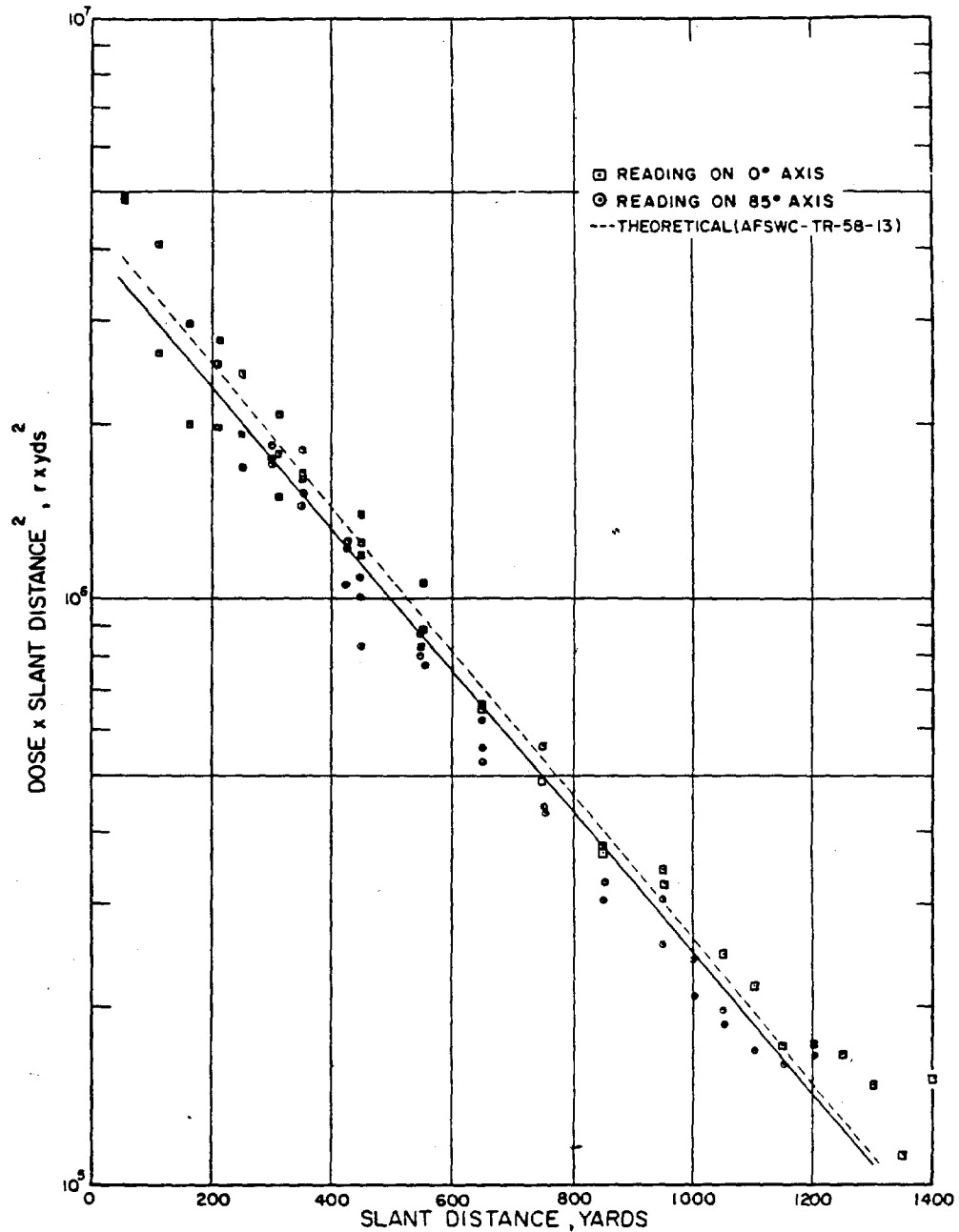
Figure 3.5 Summary of initial gamma, RD^2 versus D .
