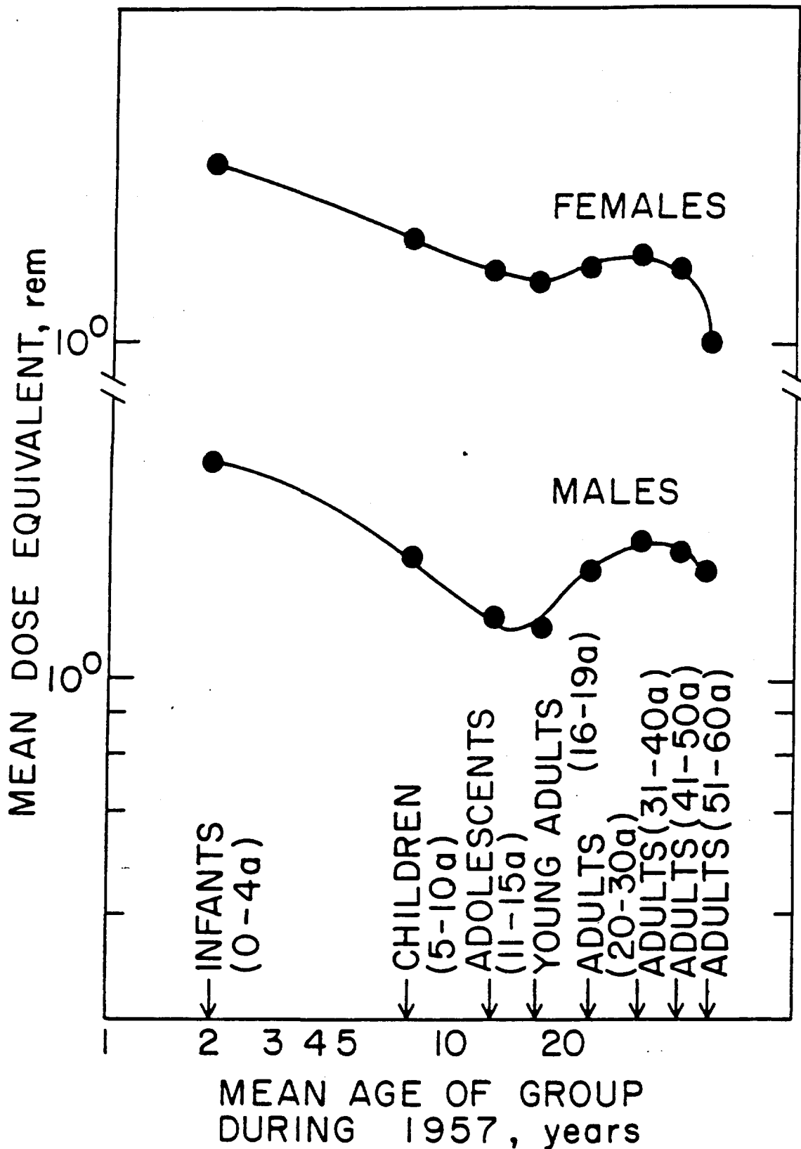
Fig. 18 ^{137}\text{Cs} Mean Dose Equivalent for Various Mid-1957 Age Groups for the Interval 1957 to 1980 at Rongelap Atoll
