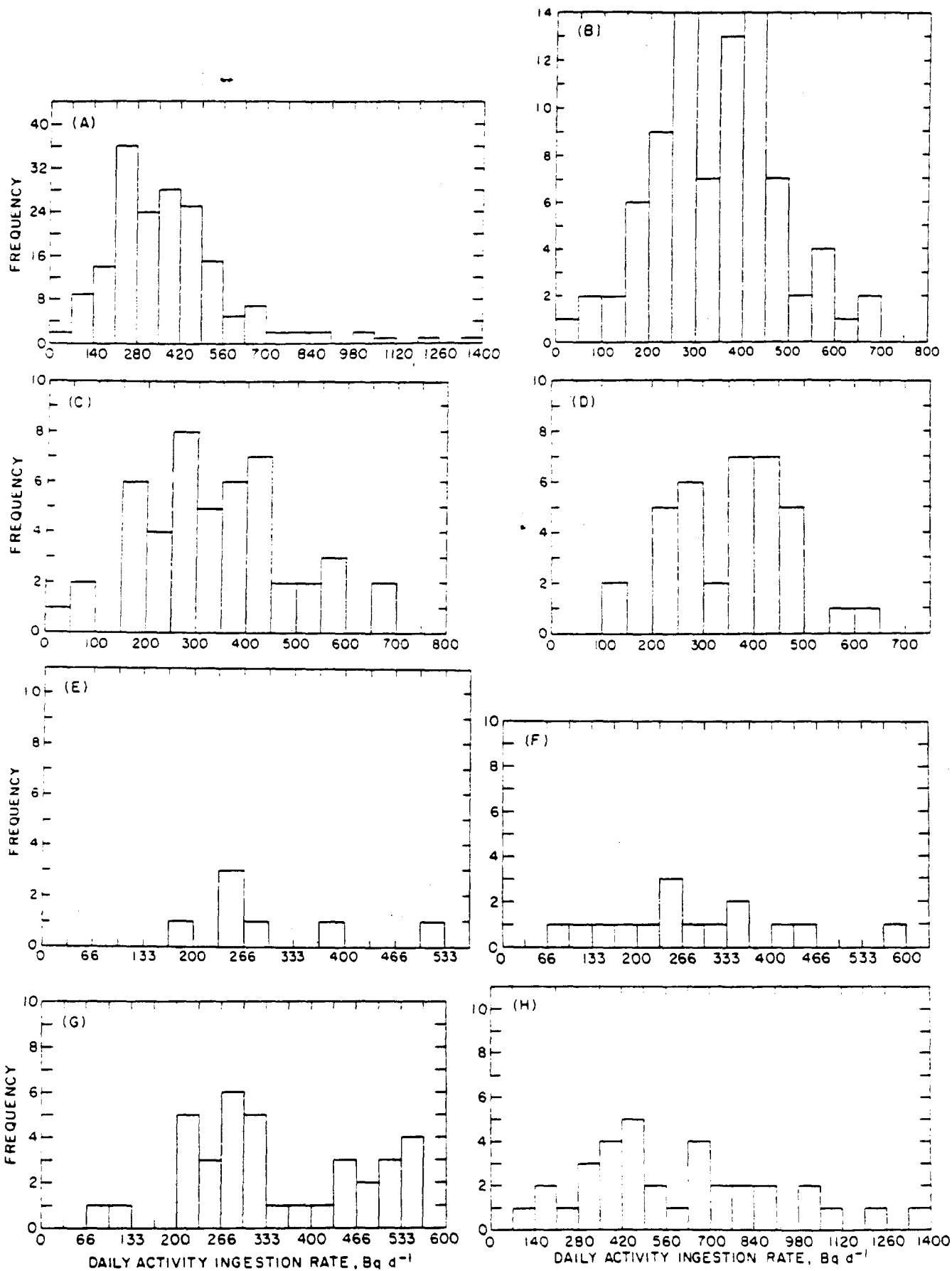
Fig. 11 137 Cs Daily Activity Ingestion Rate for (A) All Residents (B) Adults (C) Adult Males (D) Adult Females (E) Young Adults (F) Adolescents (G) Children and (H) Infants
