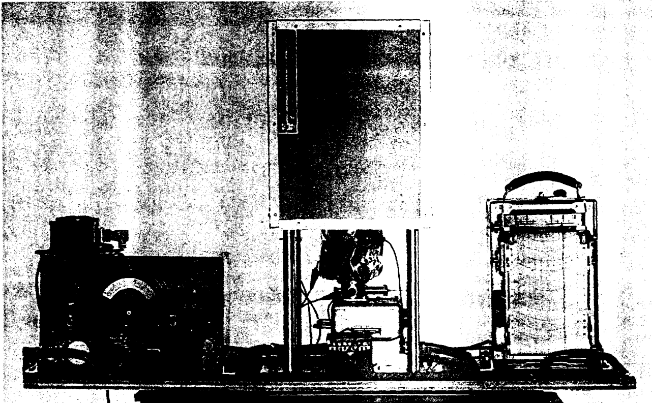
Twenty Liter Ionization Chamber and Associated Apparatus
