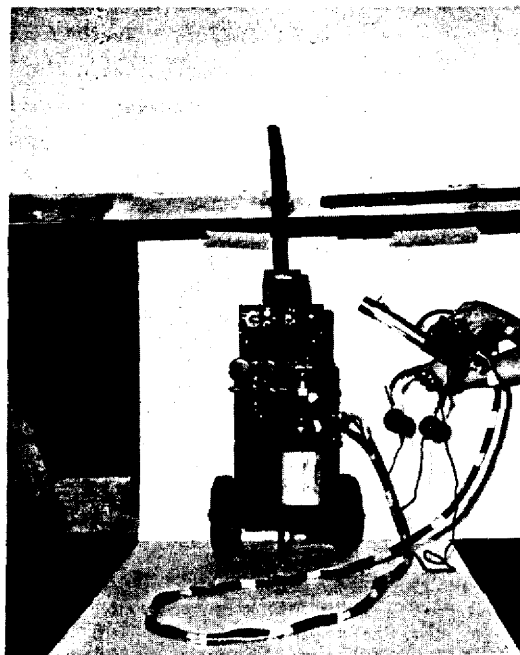
Fig. 2. A semi-portable alpha counter called "Supersnoop" used in early 1945.
