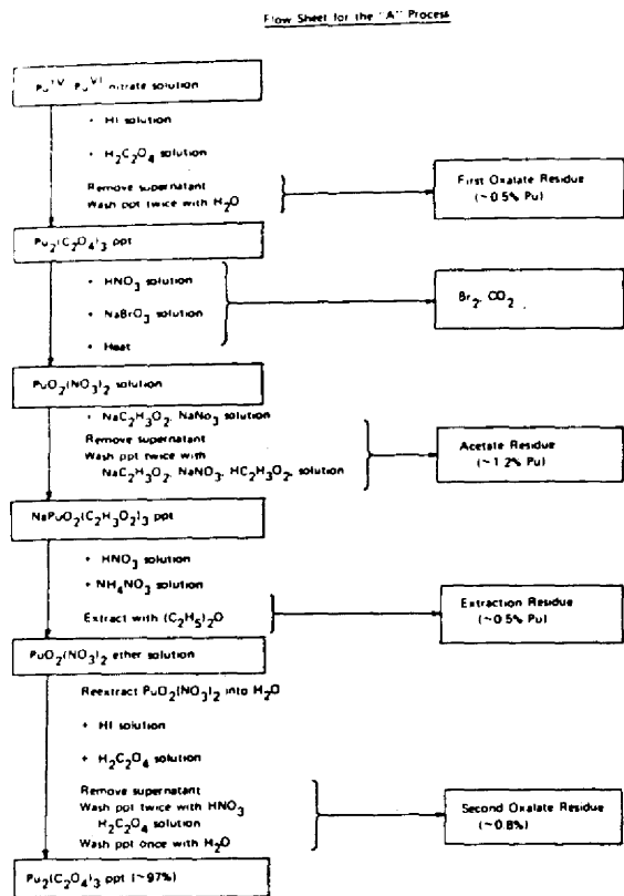
Fig. 6. Flow sheet for the purification operation. 3
