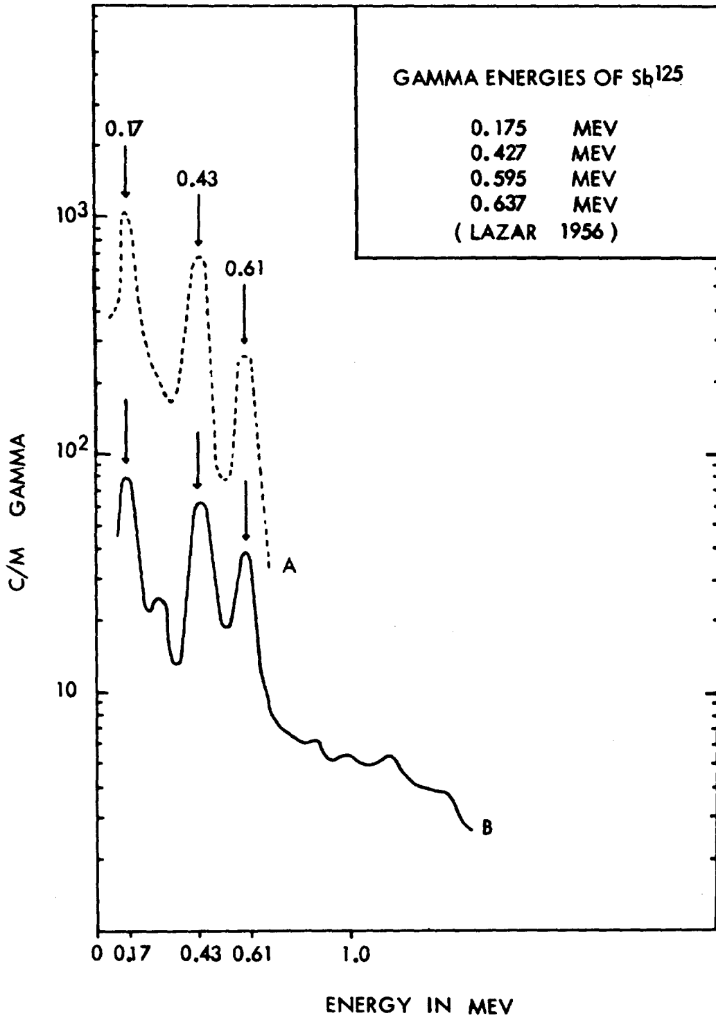
Fig. 3 (A) Gamma spectrum of the 0.1 M oxalic acid fractions from the Dowex 1 separation of the anion fraction. (B) Gamma spectrum of the antimony chemical separation.
