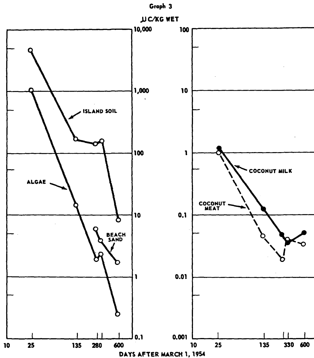
RATE OF DECLINE OF RADIOACTIVITY IN ALGAE AND SOILS AND COCONUT MEAT AND MILK AT RONGELAP ATOLL FROM MARCH 26, 1954 TO OCTOBER 23, 1955.
