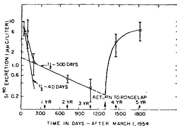
Figure 55. Urinary excretion of \text{Sr}^{90} in exposed Marshallese.
