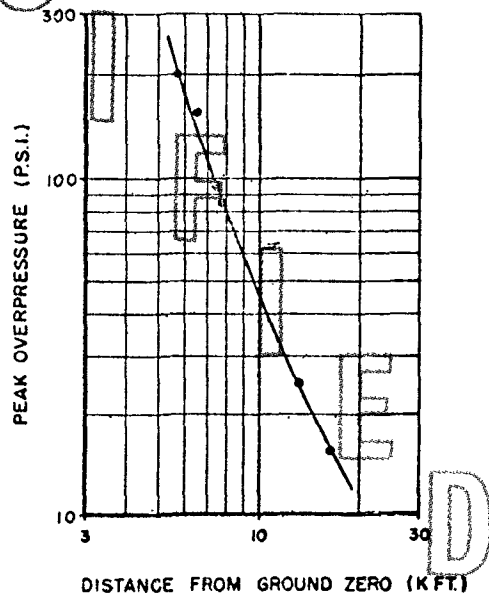
Figure 3.2 Ground surface pressure versus distance, Shot 2.
