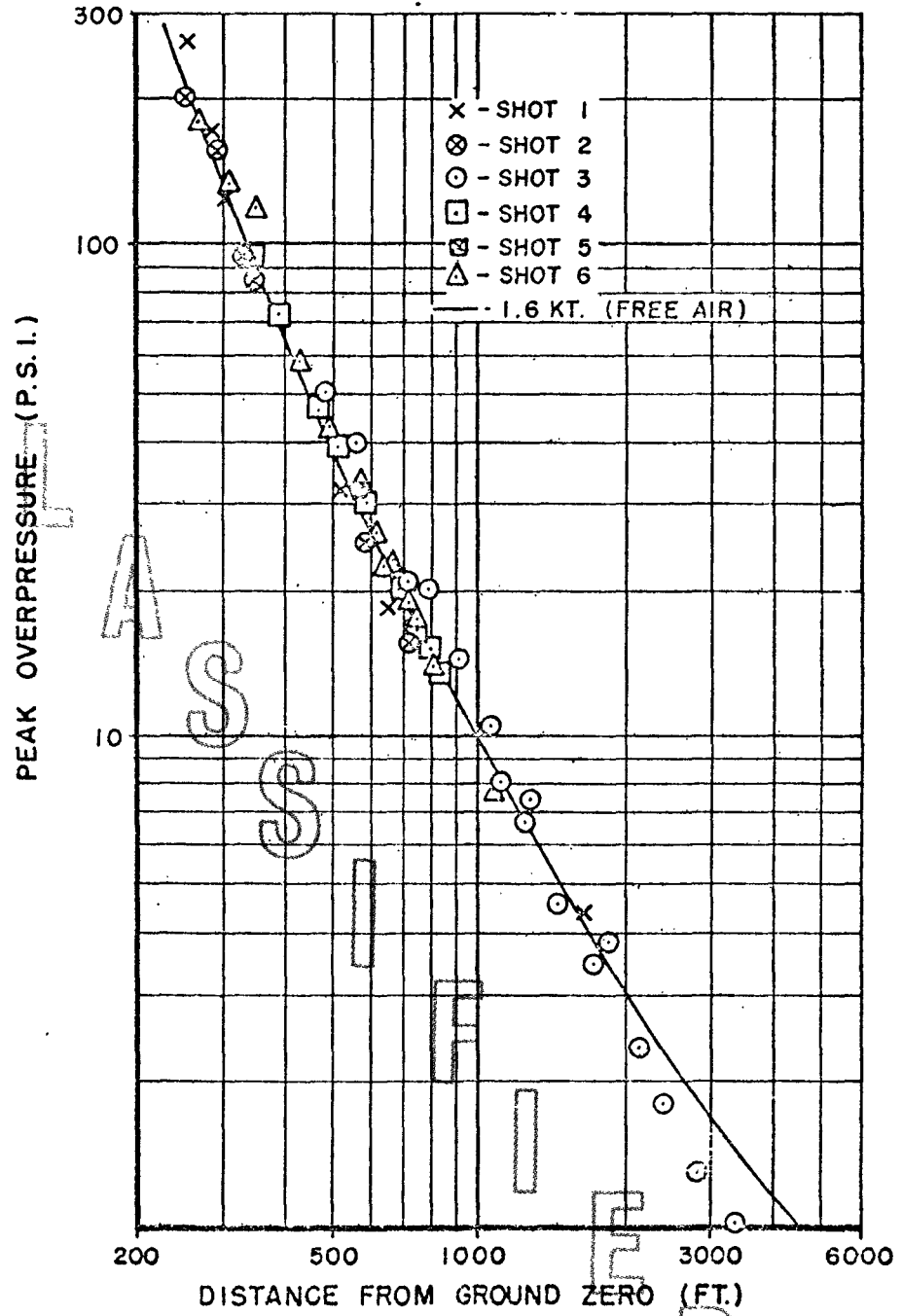
Figure 4.1 Composite ground surface pressure versus distance (scaled to 1 KT at sea level).
