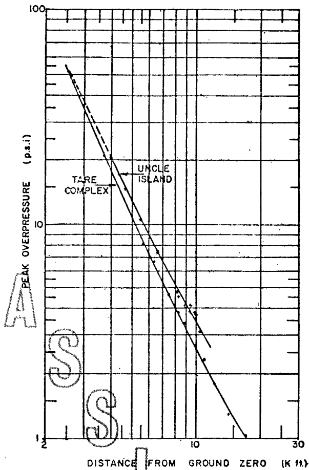
Figure 3.3 Ground surface pressure versus distance, Shot 3.
