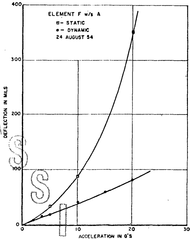
Figure E.1 Typical static and dynamic calibration curve of an air accelerometer element.
