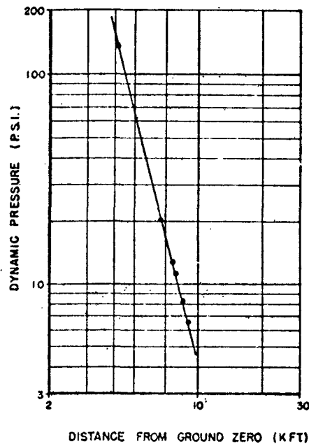
Figure 3.7 Dynamic pressure versus distance, Shot 6.
