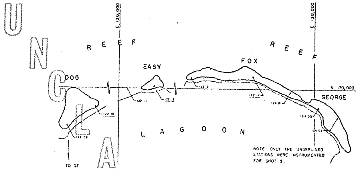
Figure 2.6 Blast line layout, Shots 4 and 5.
