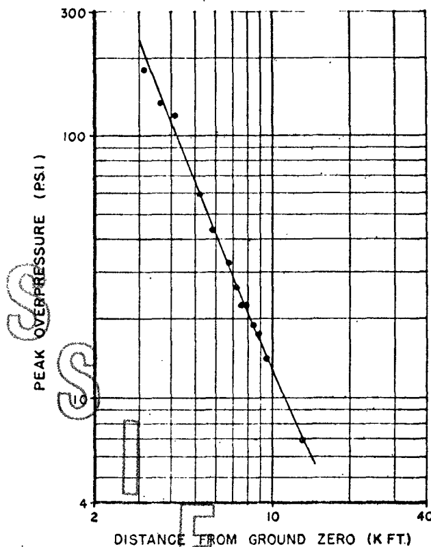
Figure 3.6 Ground surface pressure versus distance, Shot 6.
