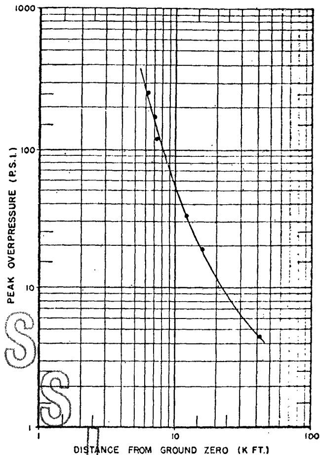
Figure 3.1 Ground surface pressure versus distance, Shot 1.
