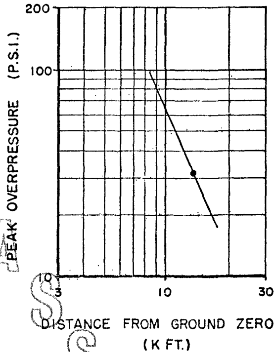
Figure 3.5 Ground surface pressure versus distance, Shot 5.
