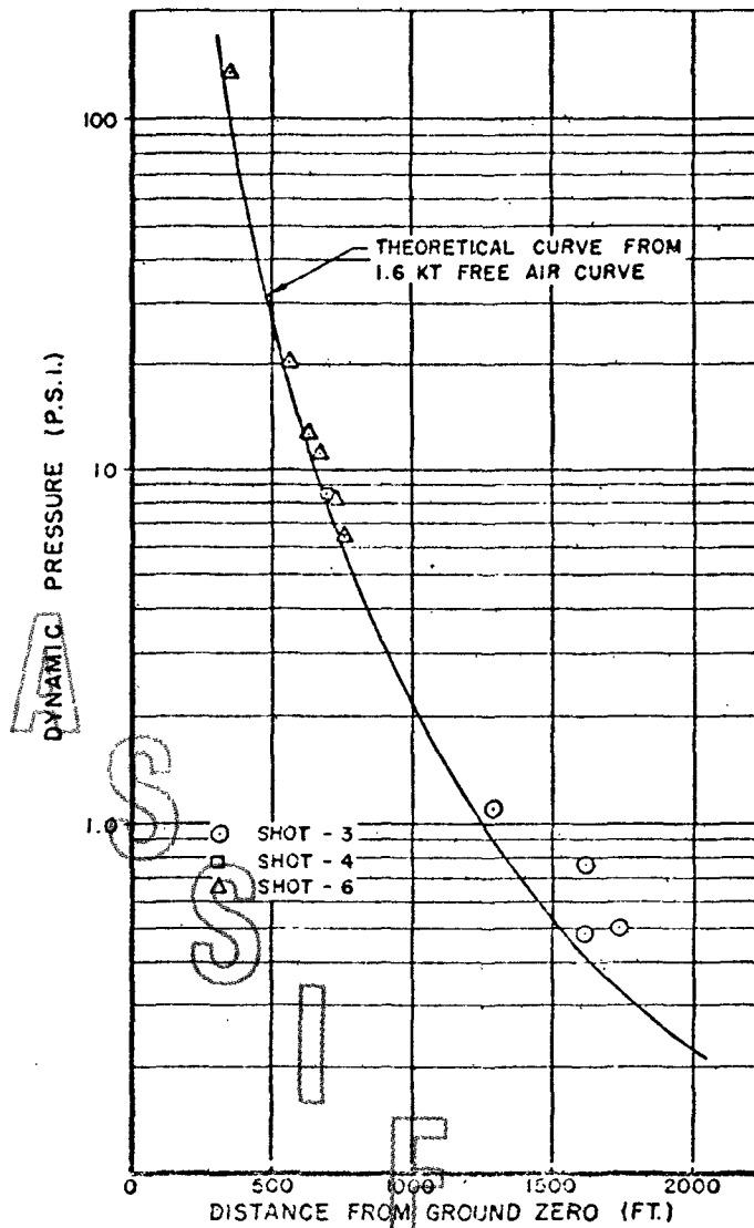
Figure 4.5 Dynamic pressure versus distance, reduced to 1 KT at sea level.
