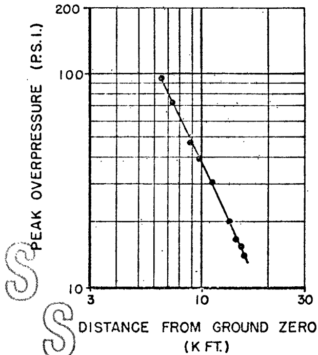
Figure 3.4 Ground surface pressure versus distance, Shot 4.
