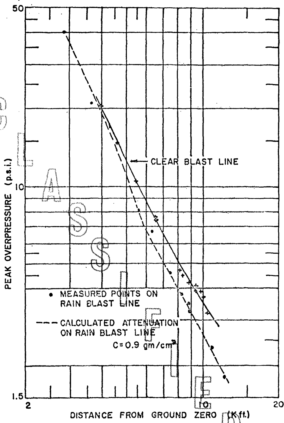
Figure 4.4 Comparison of measured and calculated attenuation of pressure, Shot 3.
