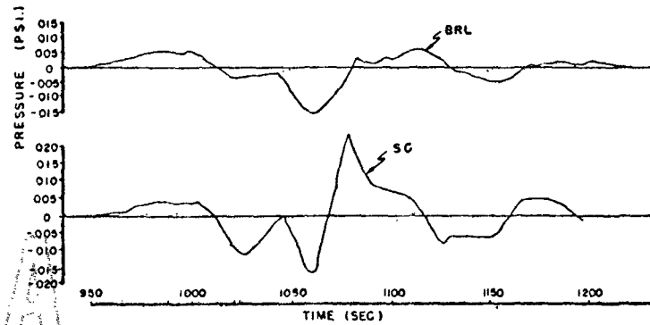
Figure F.1 Comparison of VLP, and microbarograph gage records from Site Elmer on Shot 1.
