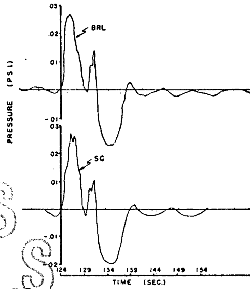
Figure F.3 Comparison of VLP, and microbarograph records from USS Curtis on Shot 3.
