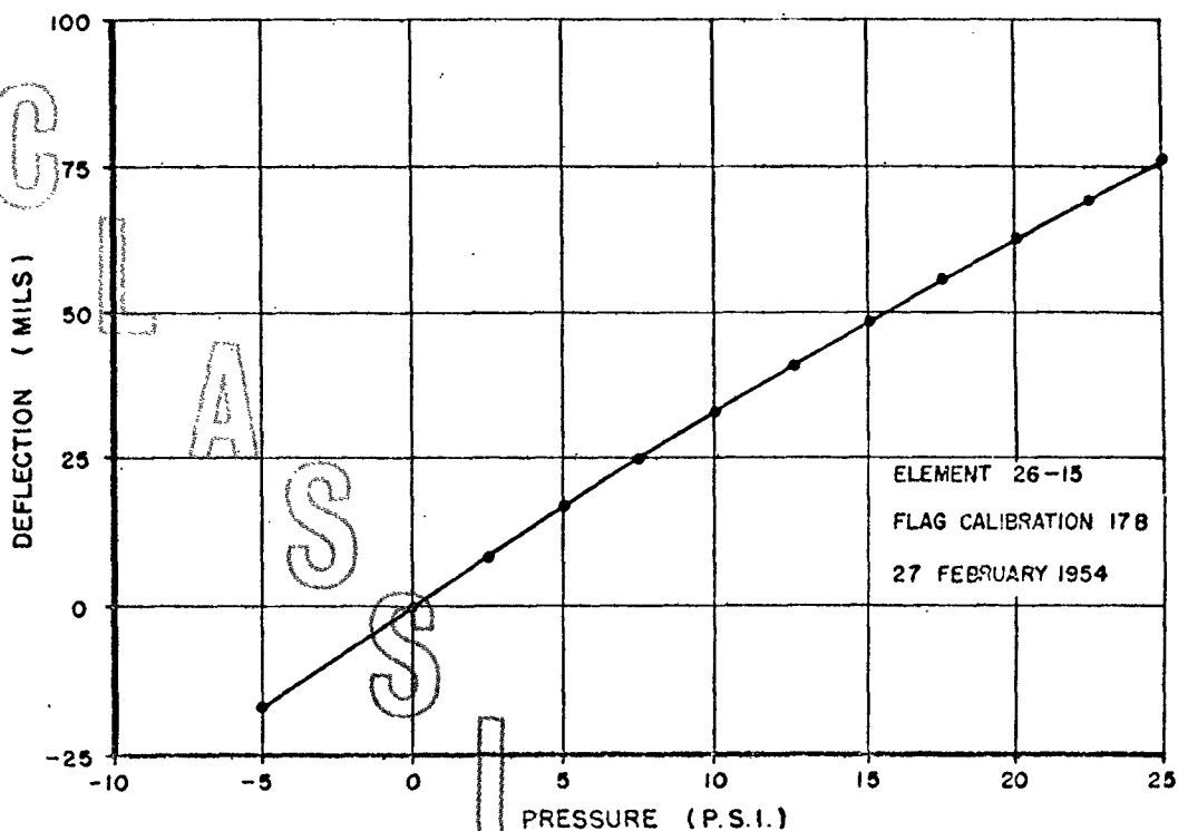
Figure B.2 Typical calibration curve for a pressure element.
