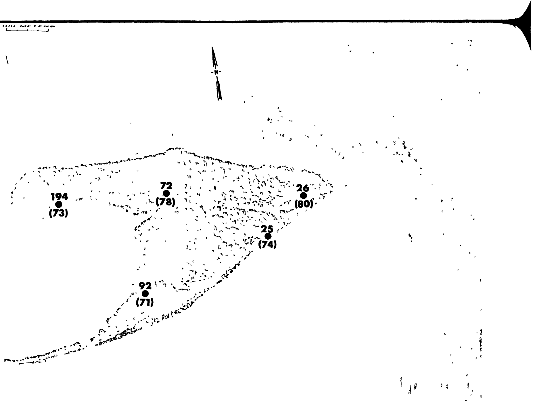
Fig. B.7.1.h. The gamma-ray exposure rates ( \mu\text{R/hr} ) measured 1 m above the ground by the LiF thermoluminescent dosimeters (TLD). The numbers shown in parentheses denote the location identification numbers.
