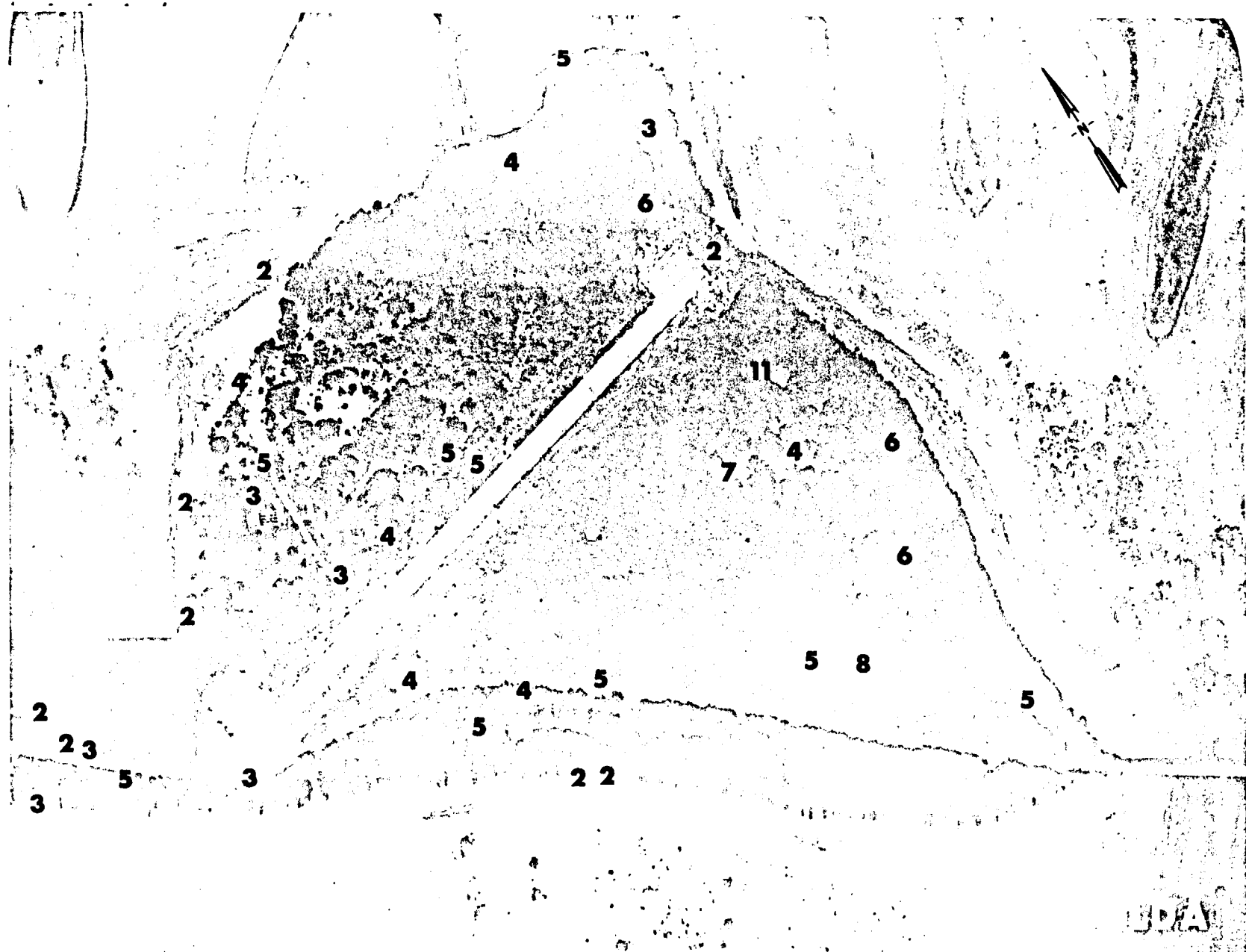
Fig. B.18.1.d. The gamma background exposure rate ( \mu\text{R}/\text{hr} ) at 1 m above the ground, measured with a portable NaI scintillation counter.
