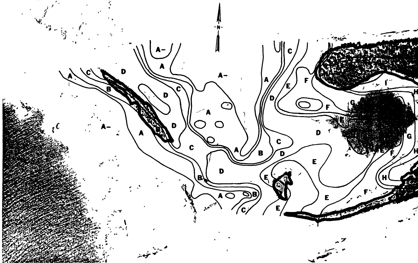
Fig. B.6.1.m. 60 Co isoexposure and isoconcentration contours. (Refer to alphabetic symbol key in this appendix.)
