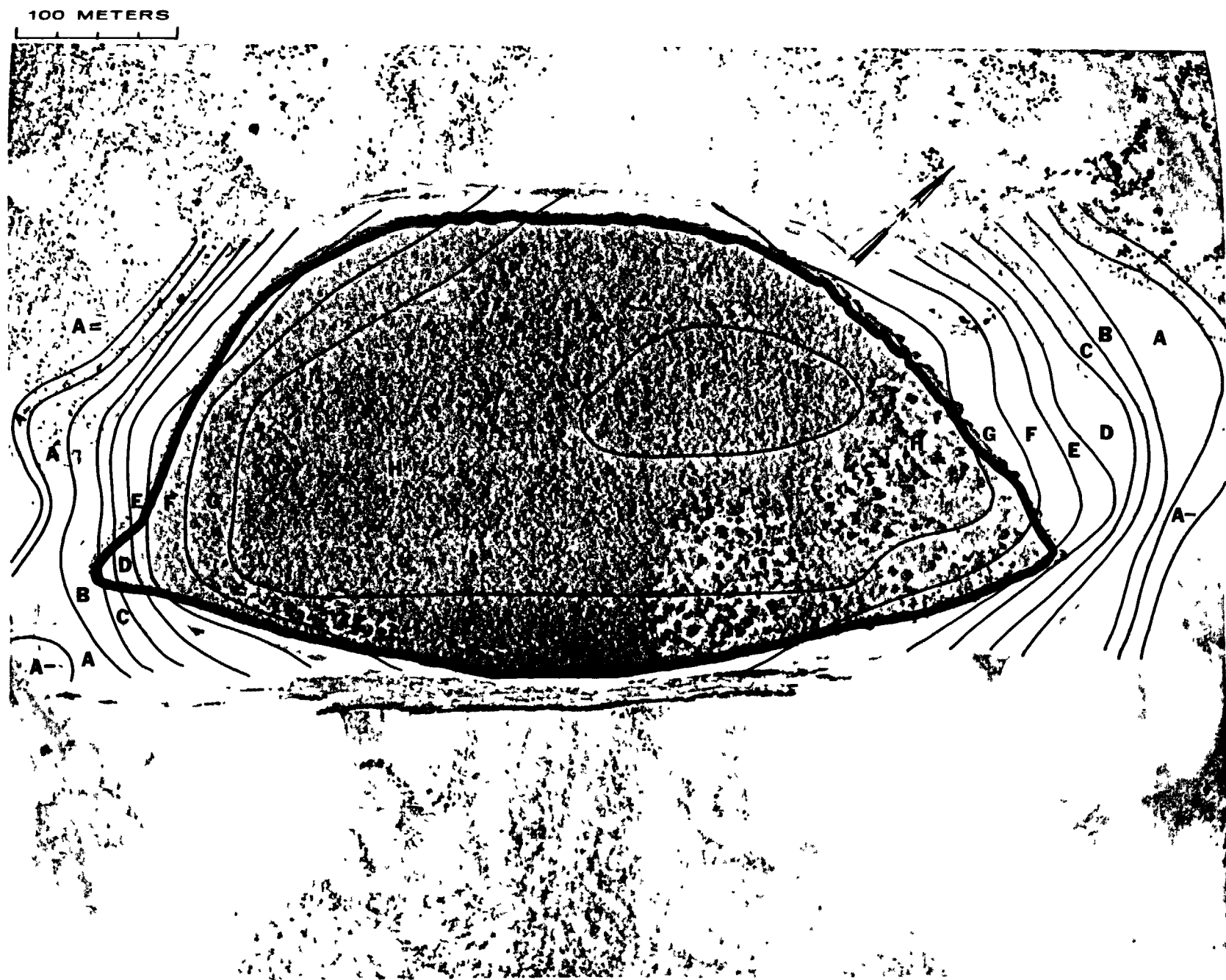
Fig. B.2.1.k. 137 Cs isosexposure and isoconcentration contours. (Refer to alphabetic symbol key in this appendix.)
