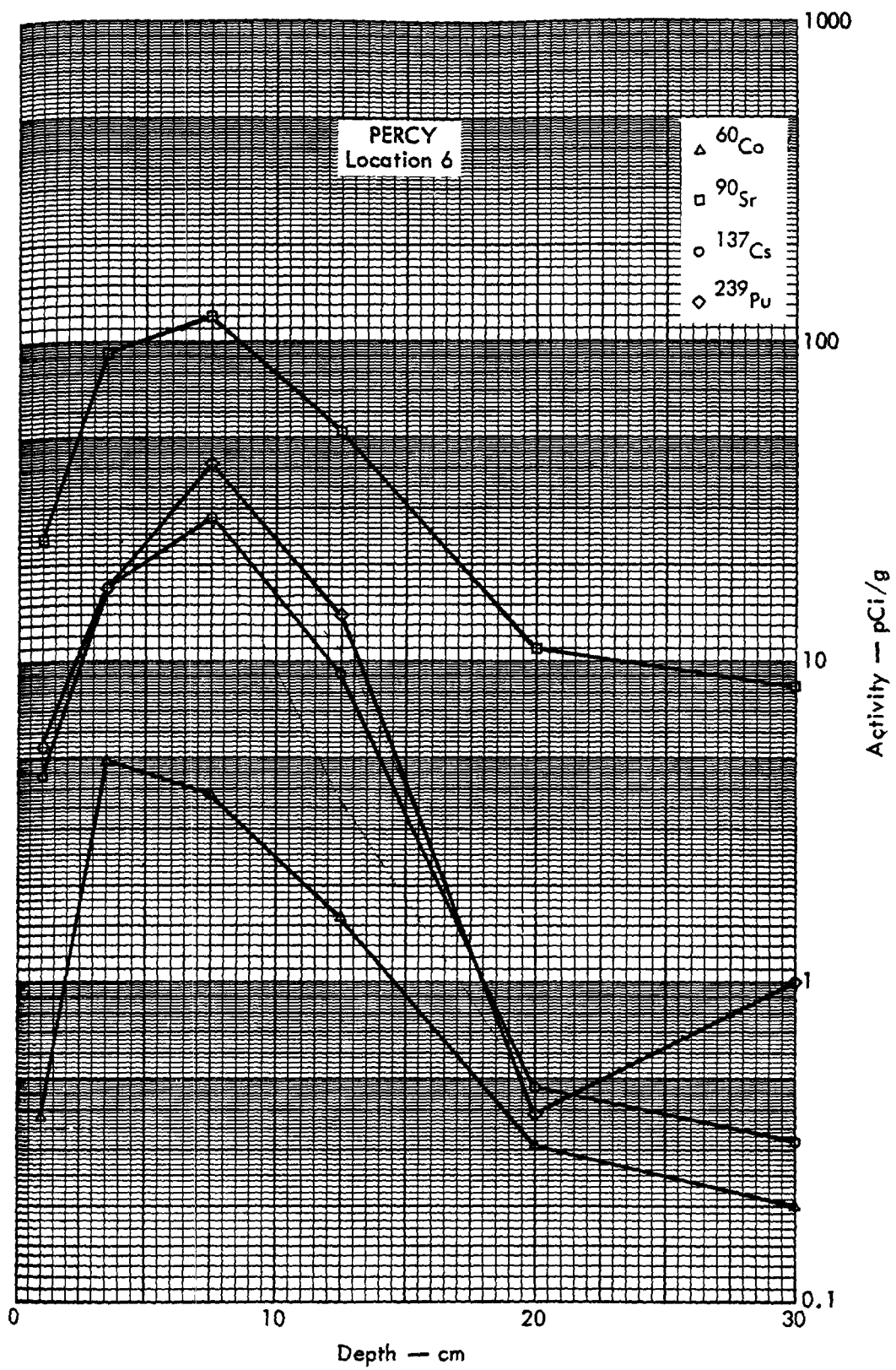
Fig. B. 11. 2a. Activities of selected radionuclides as a function of soil depth.
