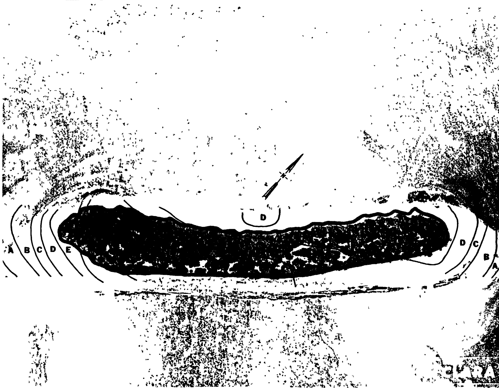
Fig. B.3.1.k. 137 Cs isoexposure and isoconcentration contours. (Refer to alphabetic symbol key in this appendix.)
