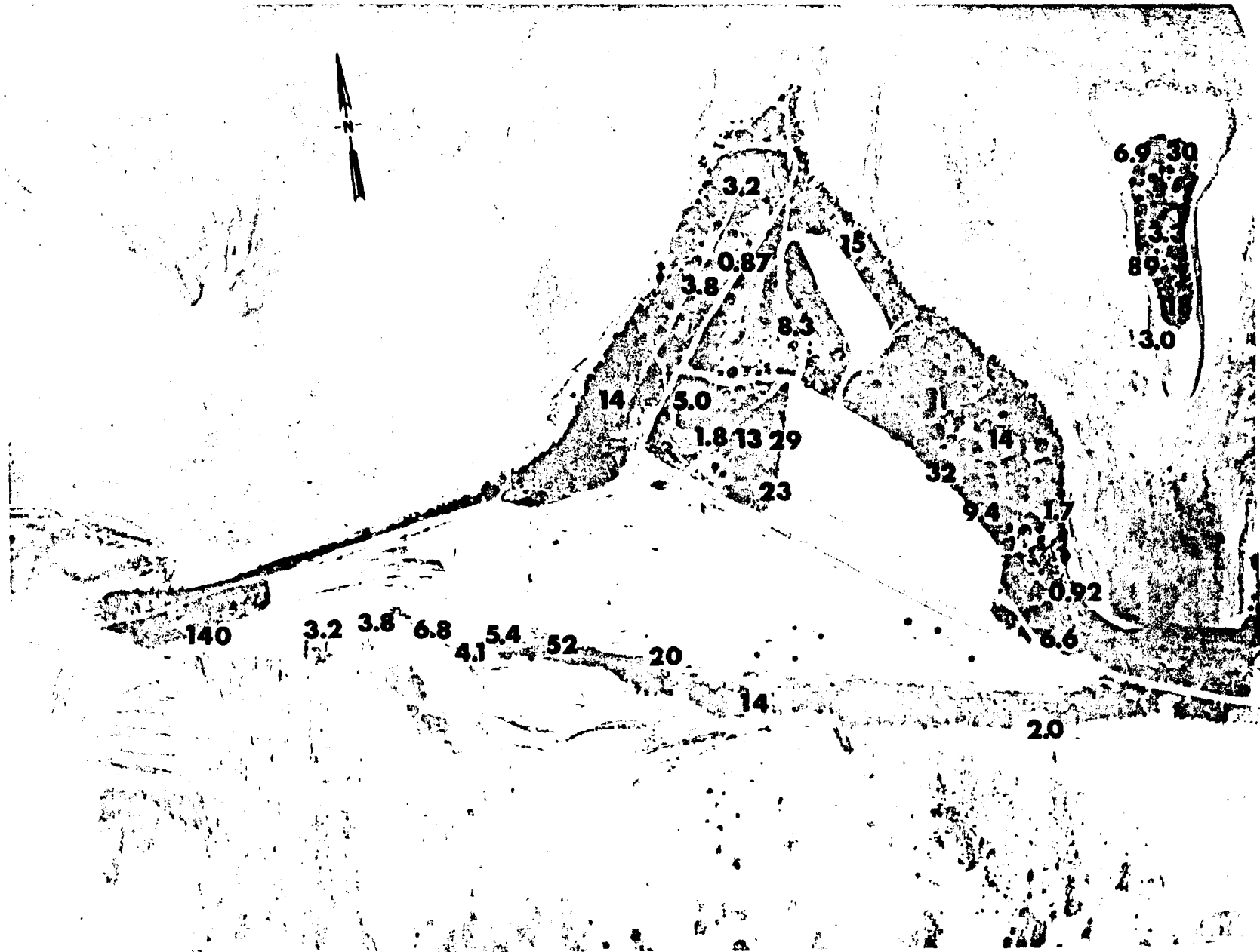
Fig. B.17.1.j. The average ^{90}\text{Sr} activities (pCi/gm) in soil samples collected to a depth of 15 cm.
