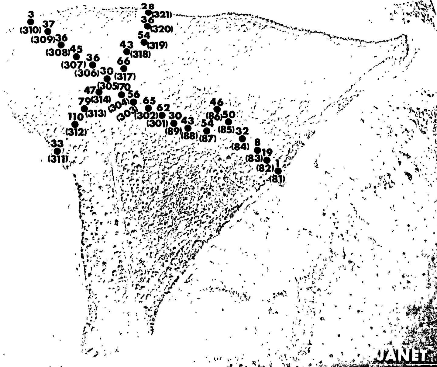
Fig. B.8.1.h. The gamma-ray exposure rates ( \mu\text{R/hr} ) measured 1 m above the ground by the LiF thermoluminescent dosimeters (TLD). The numbers shown in parentheses denote the location identification numbers.
