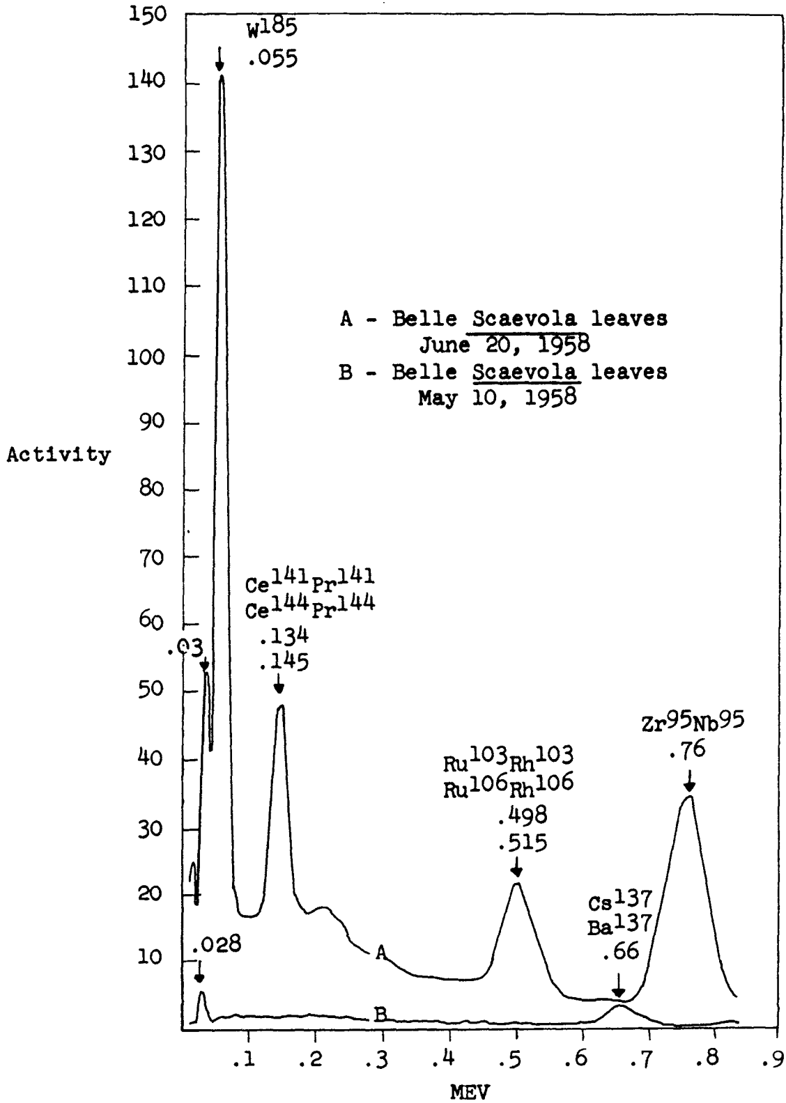
Fig. 6. Gamma spectrum curves of Scaevola leaves collected at Belle Island on May 10, 1958, prior to the W185 contamination and of those collected on June 20, 1958, after contamination. The earlier samples contained only Cs137-Ba137.
