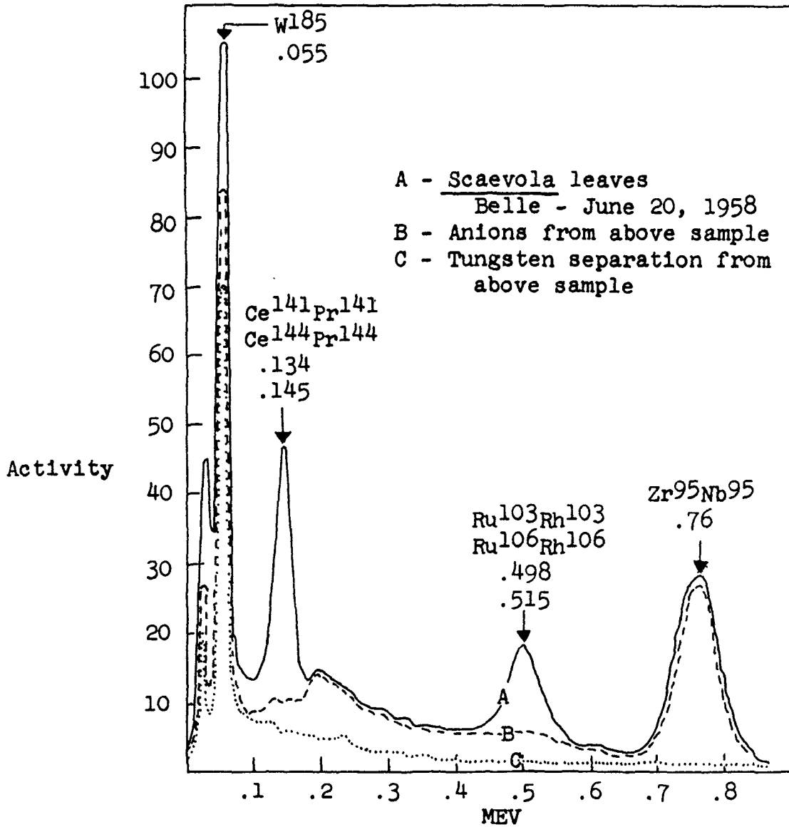
Fig. 5. Gamma spectrum curves of Scaevola leaves taken at Belle Island (Eniwetok Atoll) on June 20, 1958, and of chemical separations from the leaf samples.
