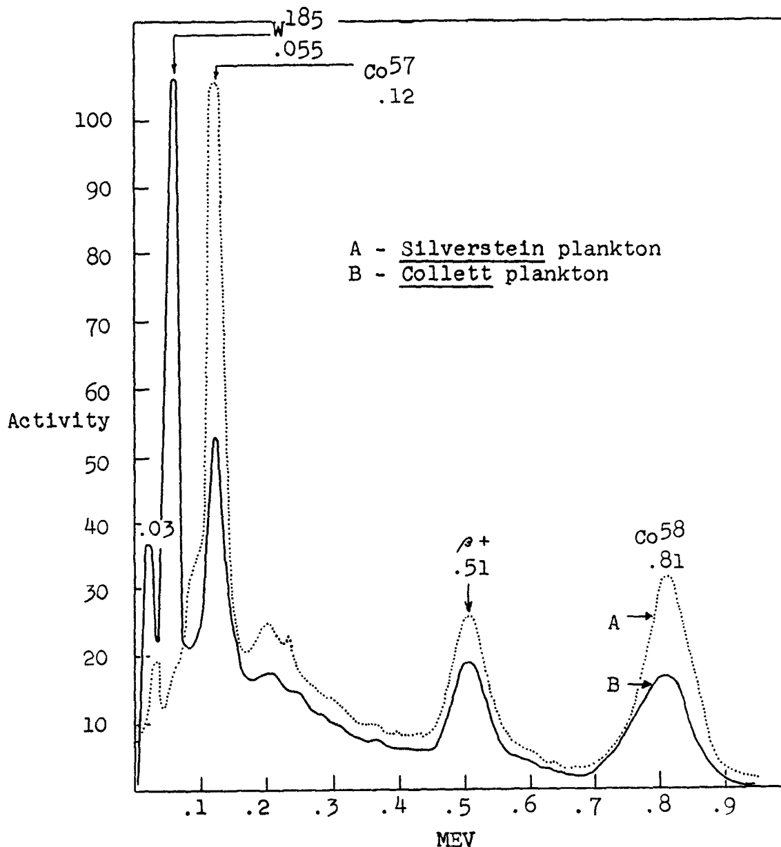
Fig. 4. Gamma spectrum curves of combined plankton samples of the Collett and of the Silverstein survey which was conducted three weeks later. W^{185} was present at a high level in the plankton from the Collett survey but was absent in the plankton from the Silverstein survey. The Collett samples contained higher levels of radioactivity than did the Silverstein samples and the gamma curves are not indicative of the relative gamma activity in the two samples.
