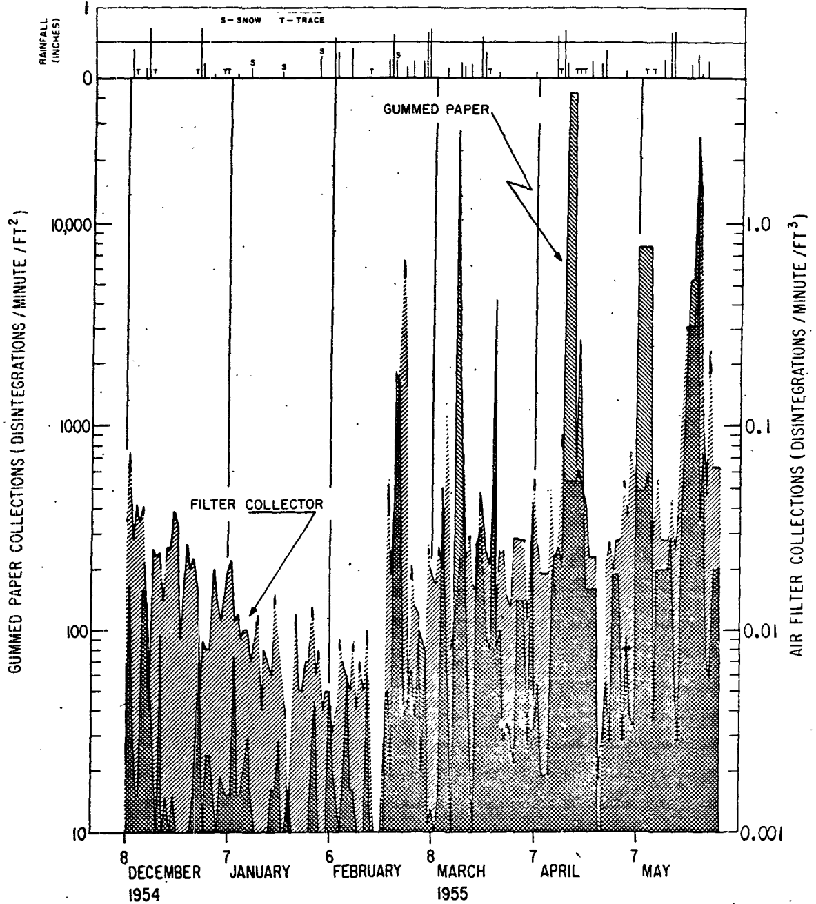
Fig. 1 - Comparison of daily concentrations of fission products collected by gummed paper and air filters
