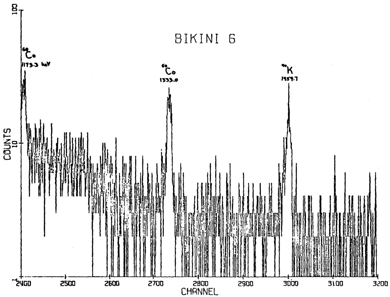
Figure 8d. Ge(Li) spectrum of soil sample taken from Bikini Island, Pit 6, 0 Transect, Location 5.
