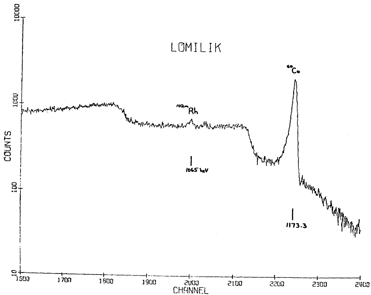
Figure 11c. Ge(Li) spectrum of soil sample taken from Lomilik Island, Aomen-Iroj Complex.
