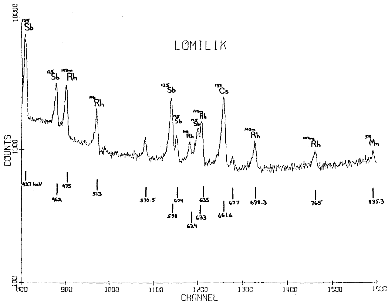
Figure 11b. Ge(Li) spectrum of soil sample taken from Lomilik Island, Aomen-Iroij Complex.
