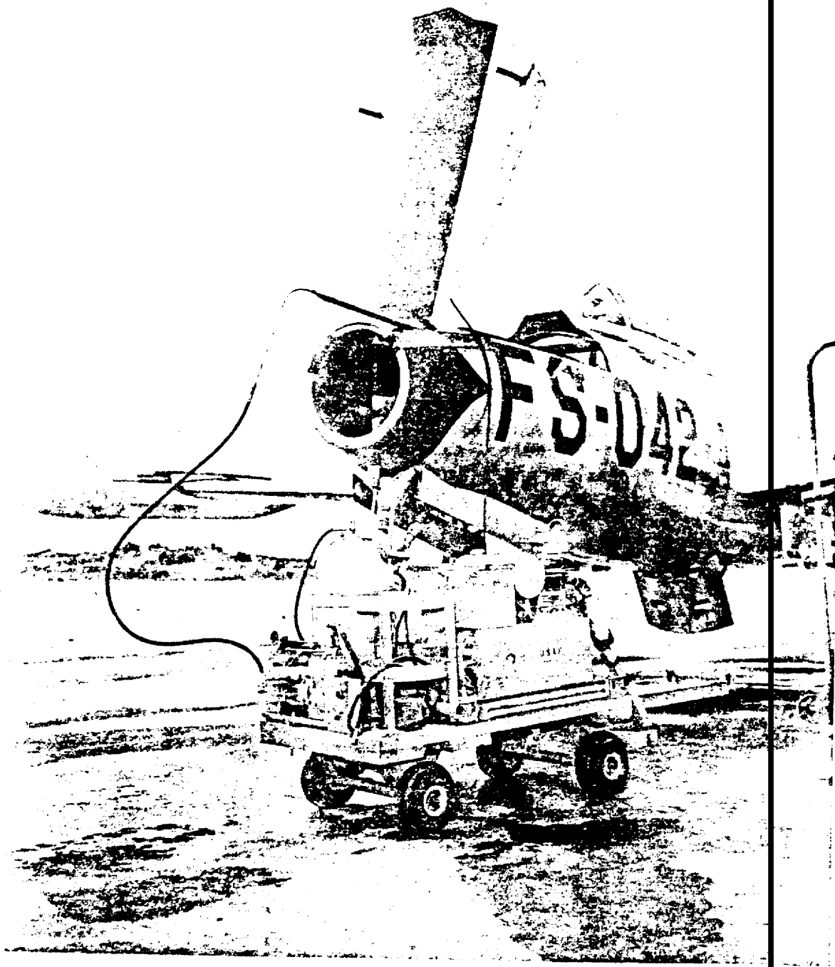
Figure 34. Removal of gas sample from "snap-bag" through sampling probe, CASTLE.
