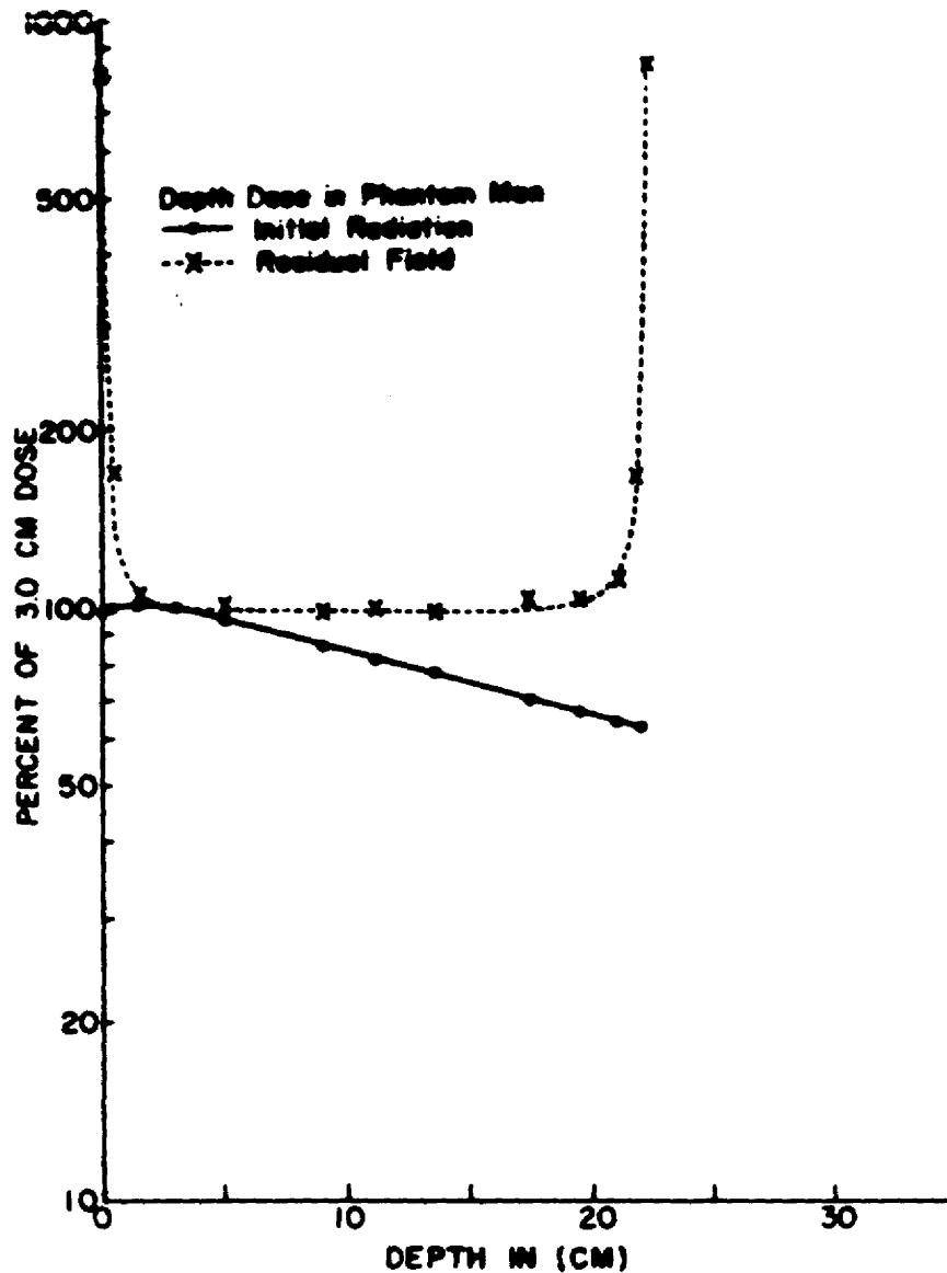
FIGURE 1.5—Comparison of depth dose curves in a manometric phantom man, of the initial atomic bomb gamma radiation and of gamma radiation from a planar field of fission products deposited on soil after an experimental nuclear detonation.
