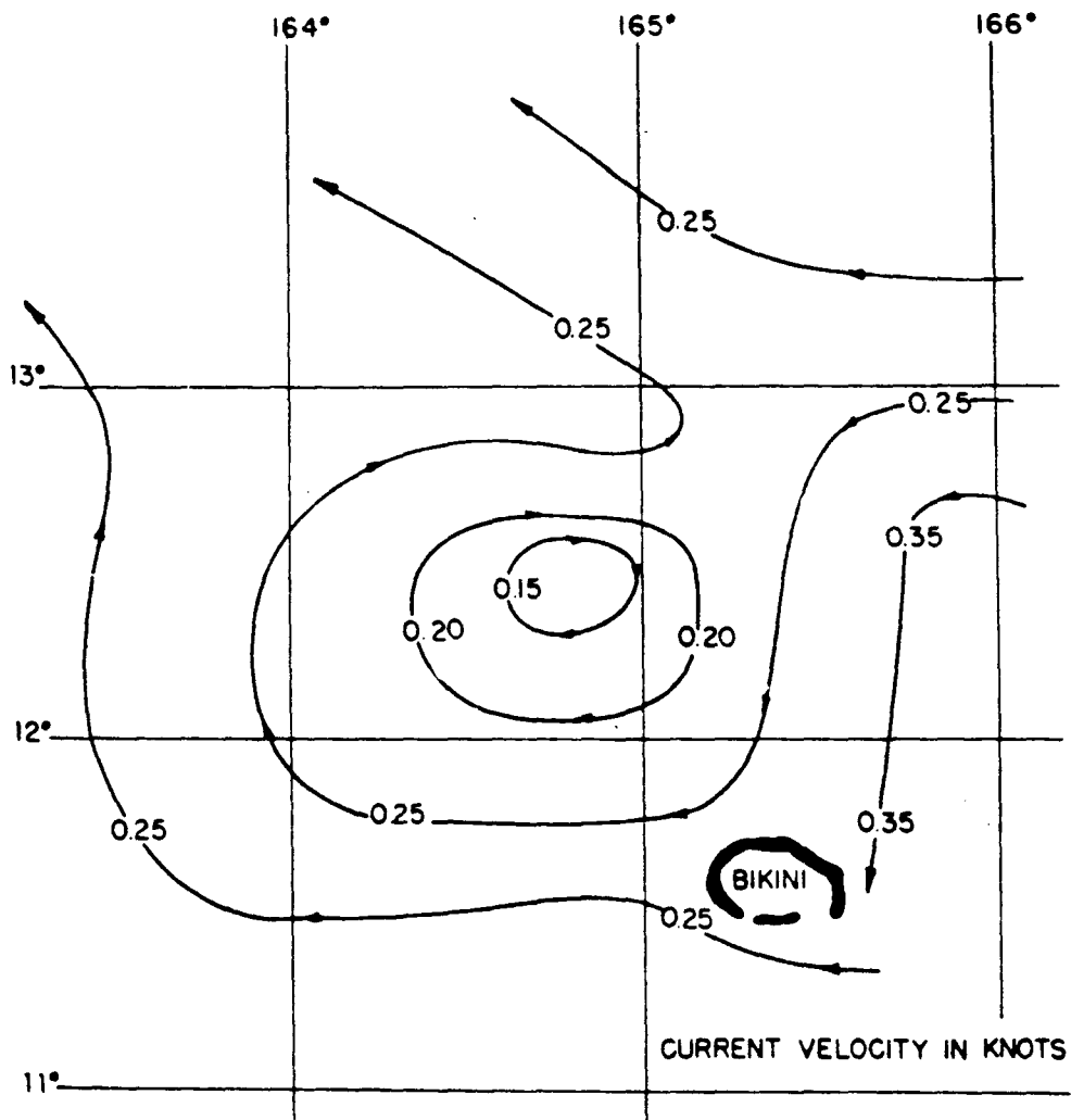
Figure 2.26 Deduced streamlines of ocean currents, Shot Flathead.
