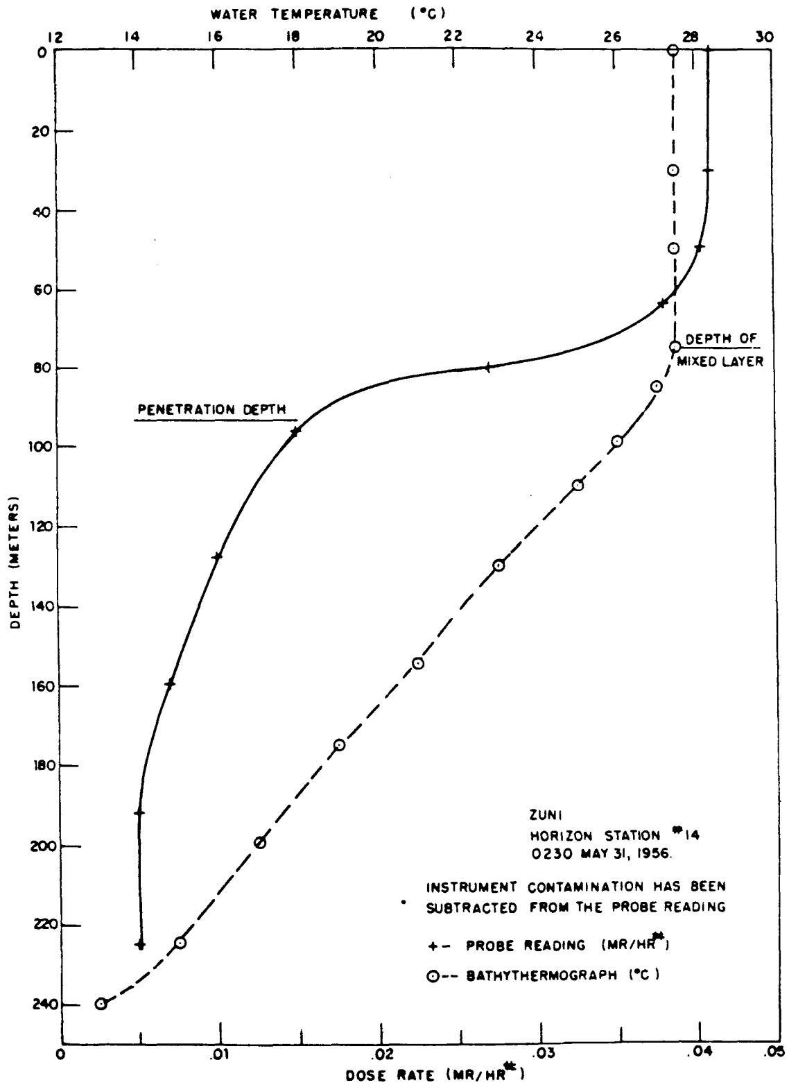
Figure 2.16 Comparison of dose rate and temperature versus depth, Shot Zuni.
