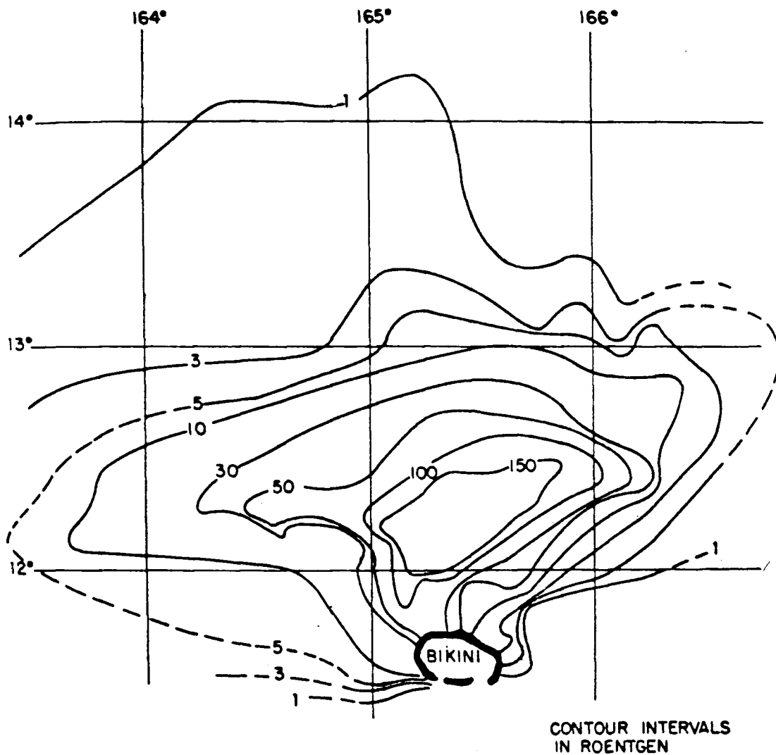
Figure 2.37 Accumulated dose (time of arrival to H+50), Shot Zuni.
