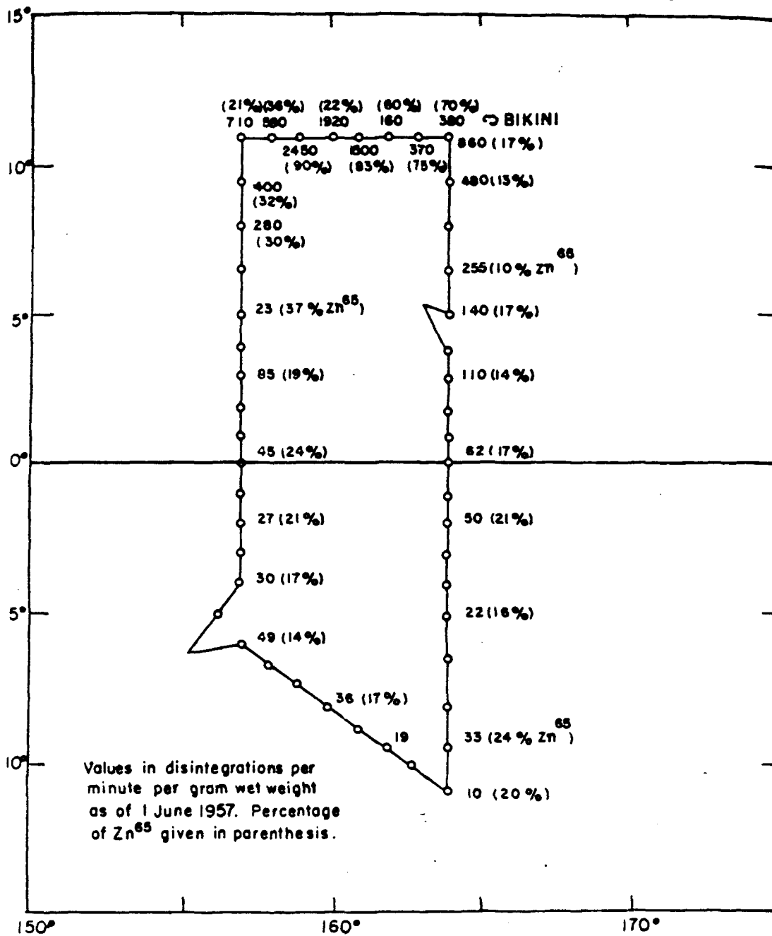
Figure 5.5 Distribution of plankton radioactivity across Equatorial Pacific.
