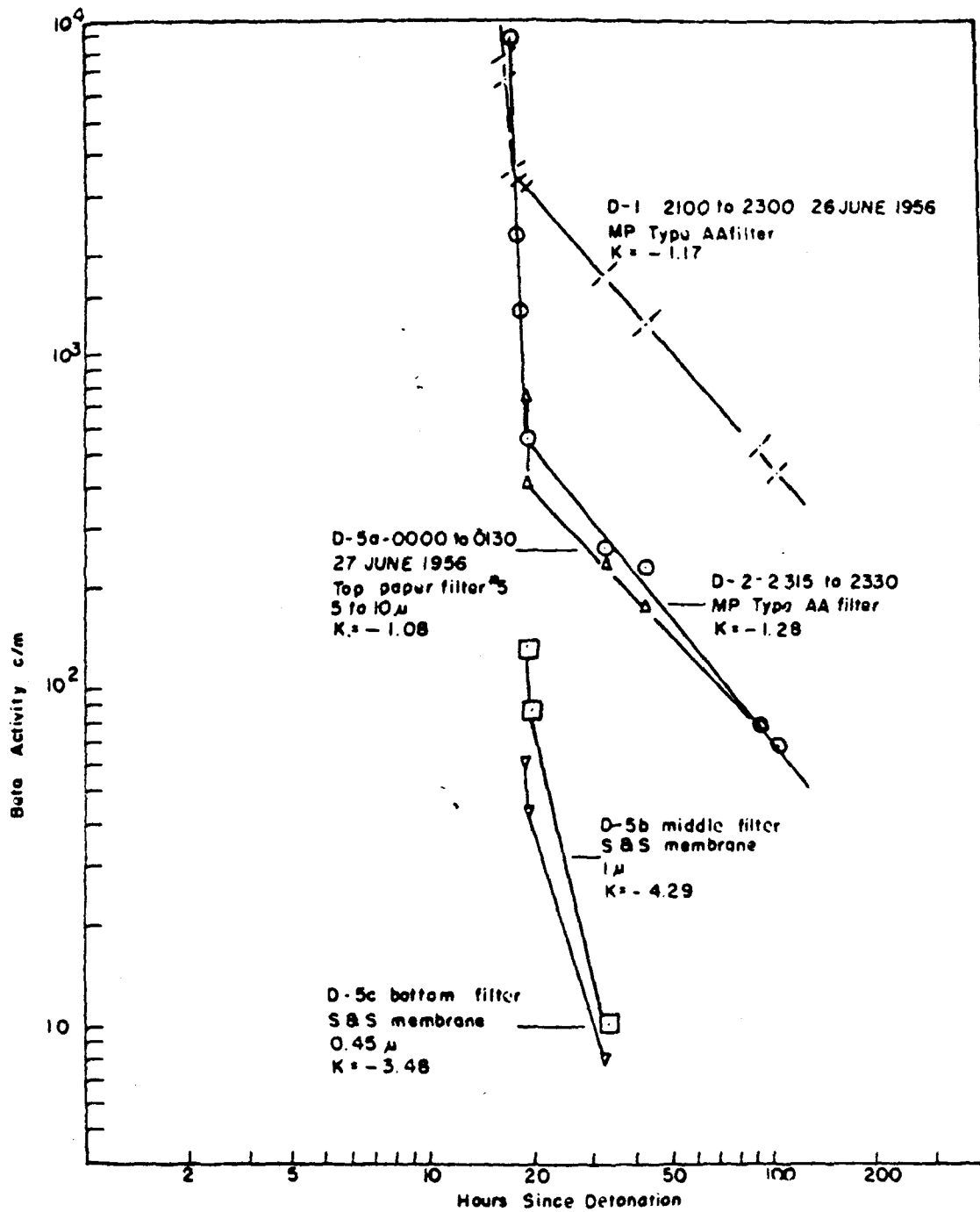
Figure 5.2 Decay curves for Shot Dakota air samples.
