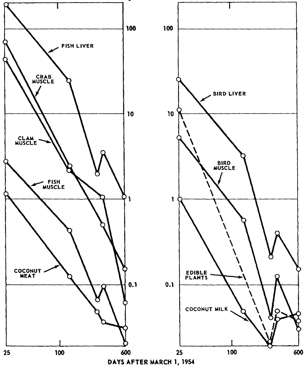
RATE OF DECLINE OF RADIOACTIVITY IN FOOD ITEMS FROM COLLECTIONS AT RONGELAP ATOLL BETWEEN MARCH 26, 1954 AND OCTOBER 22-23, 1955. (AFL)
