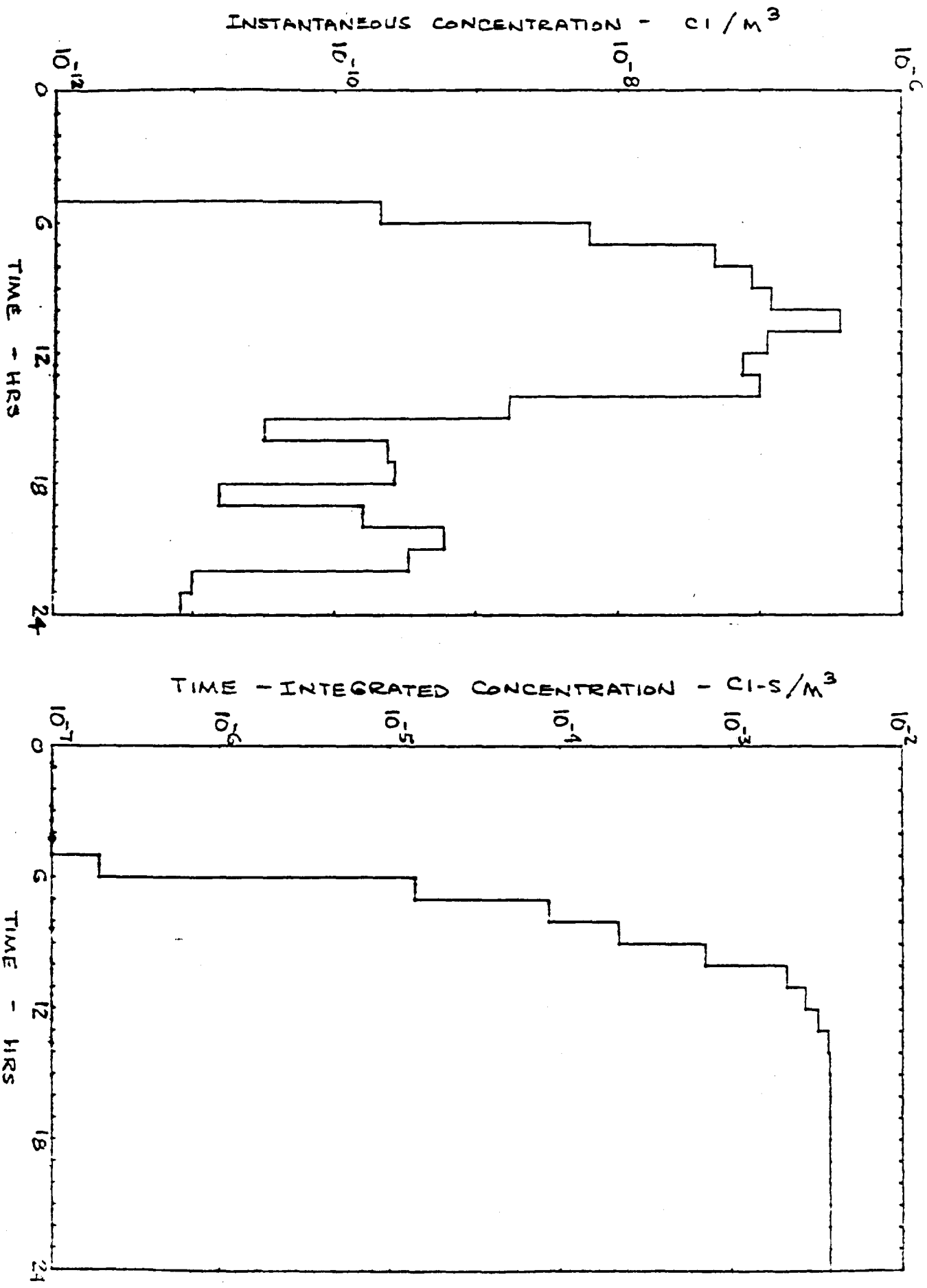
Figure 4b, Same as Fig. 4a, except nuclide is Iodine-131.
