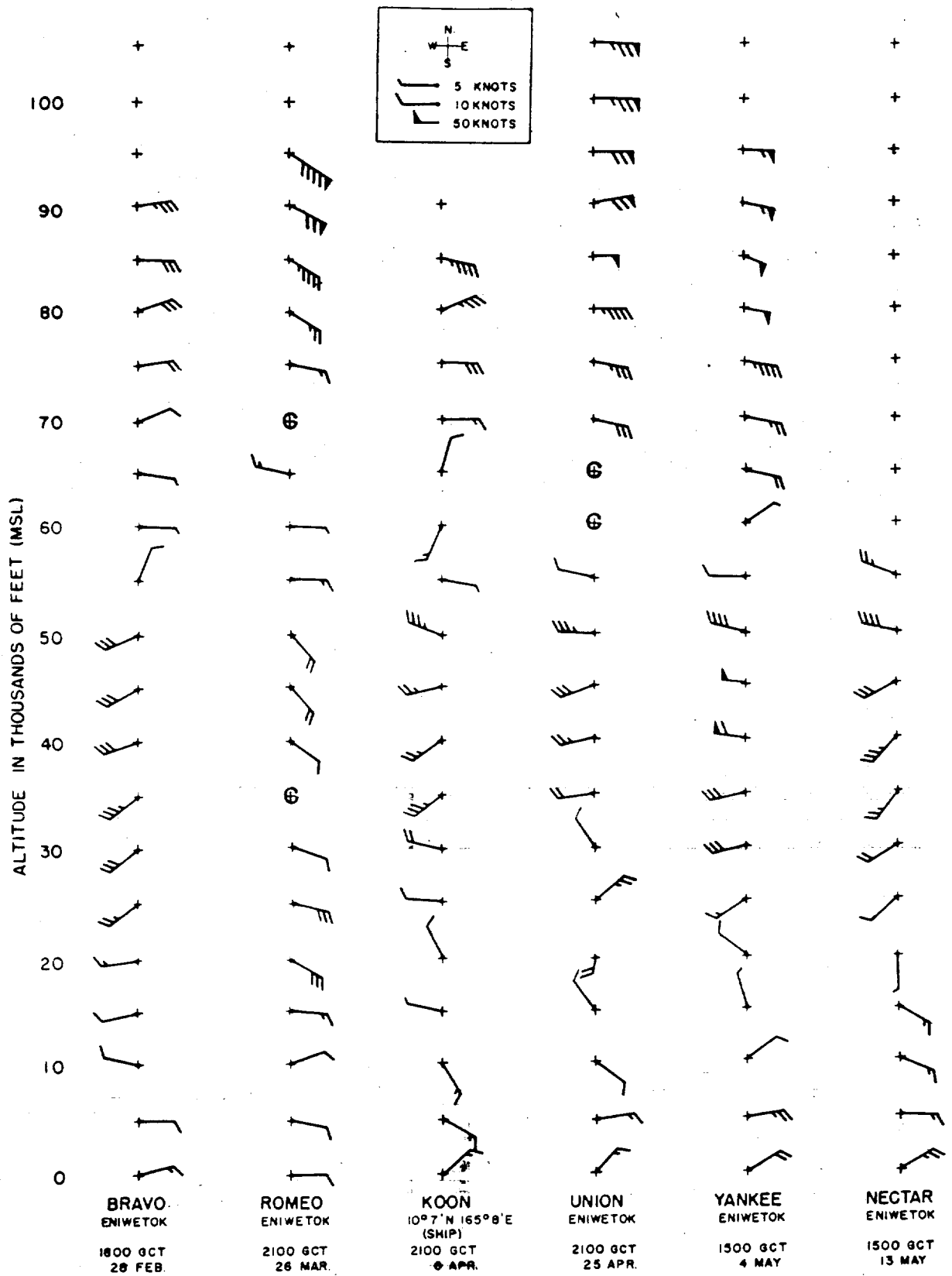
FIGURE 2.1 WINDS ALOFT FOR CASTLE EVENTS
