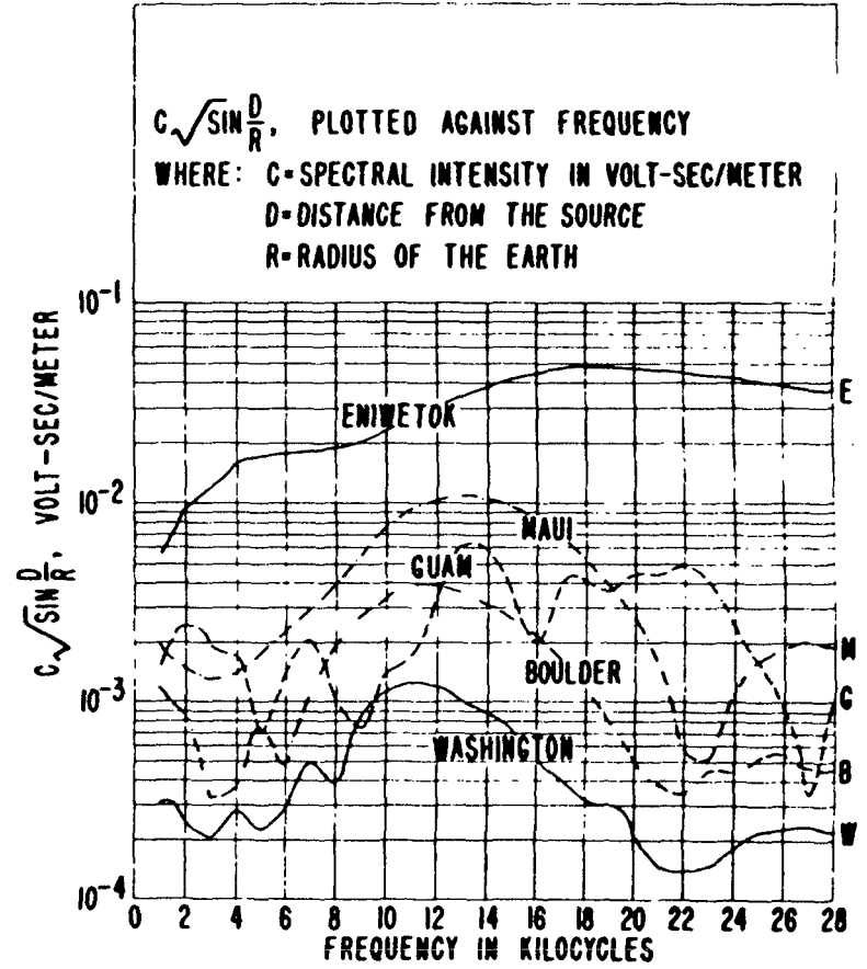
Figure 15 Spectral intensity, as a function of frequency, for Shot 3 as received at selected NBS stations.
