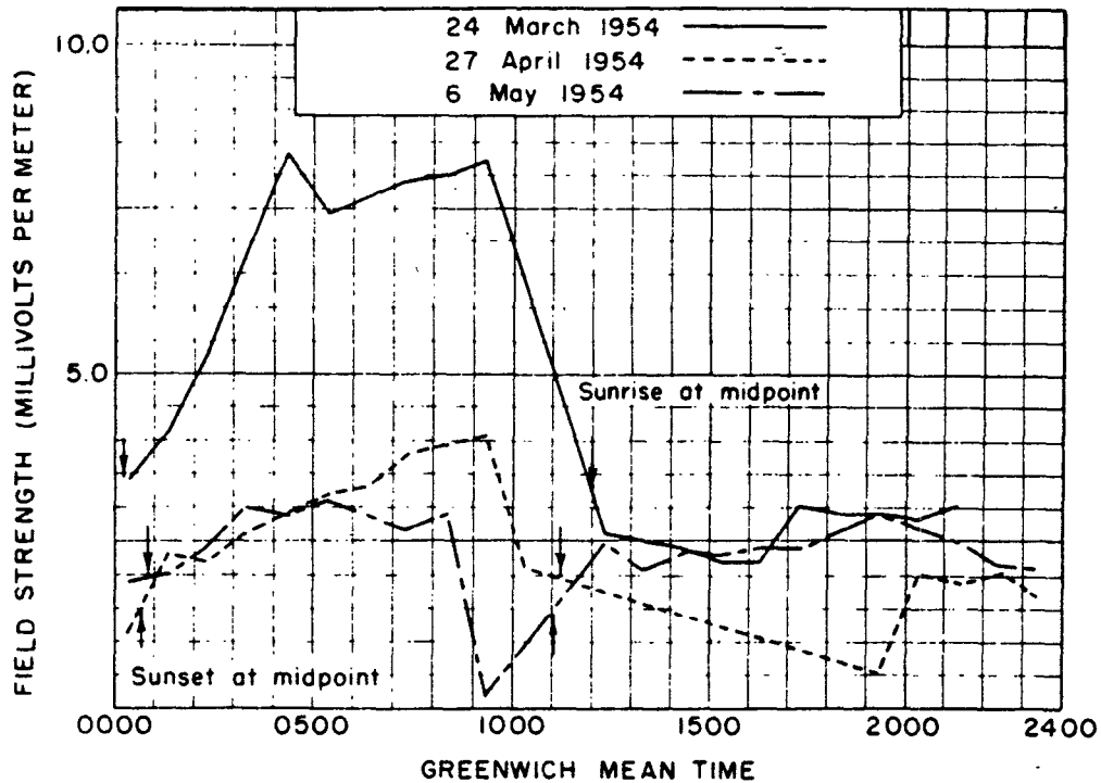
Figure 21 Plot of the field strength of NSS as measured by DRL at Austin, Texas.
