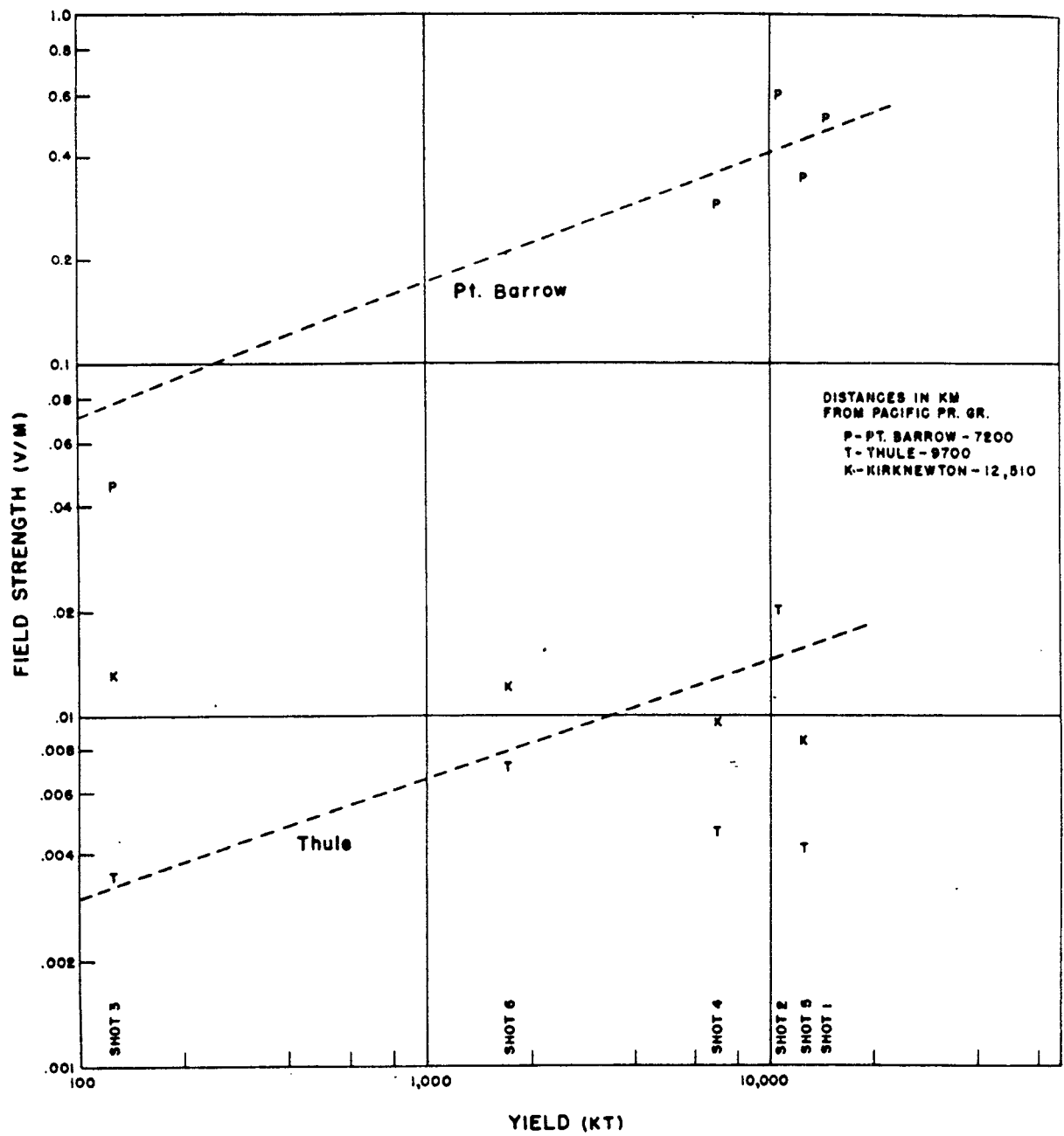
Figure 6 Plot of selected Castle data showing the relationship between peak field strength and yield on a north-south path. Probable curves, drawn by inspection, are shown for Ft. Barrow and Thule.
