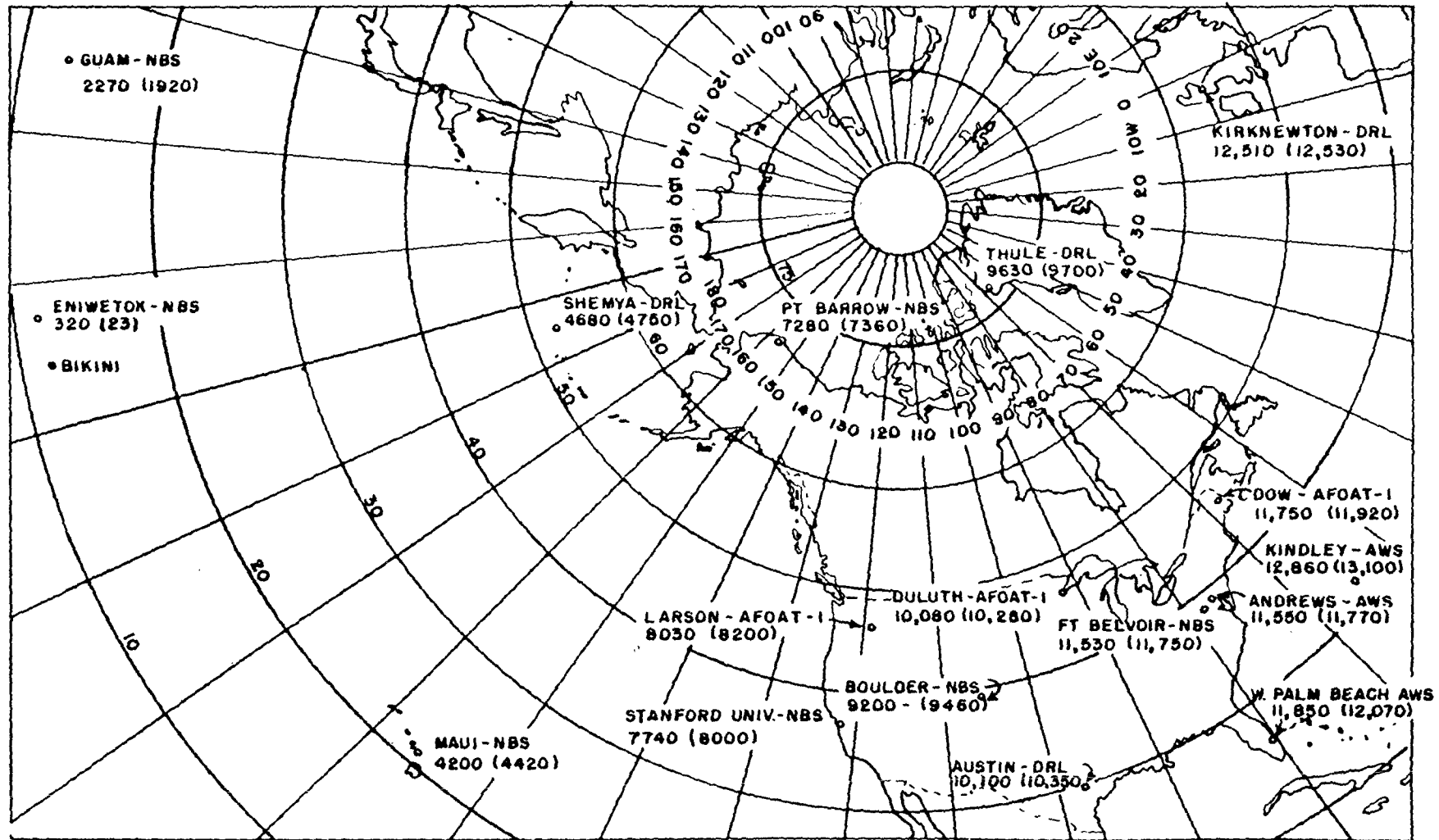
Figure 4 Pertinent information on Castle electromagnetic stations. Information includes station locations; sponsoring agencies; and approximate distances, in kilometers, from Bikini and Eniwetok (figures in parentheses). NBS, National Bureau of Standards; DRL, Defense Research Laboratory; AWS, Air Weather Service; AFOAT-1, Air Force Office for Atomic Energy.
