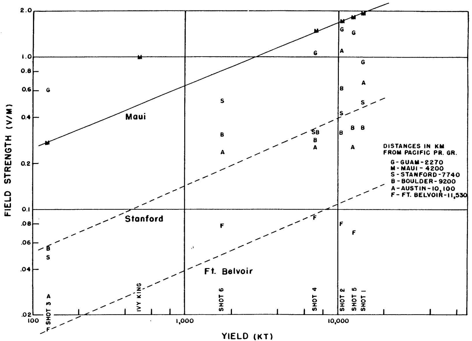
Figure 5 Plot of selected Castle data showing the relationship between peak field strength and yield on an east-west path. Probable curves, drawn by inspection, are shown for Maui, Stanford University and Ft. Belvoir.
