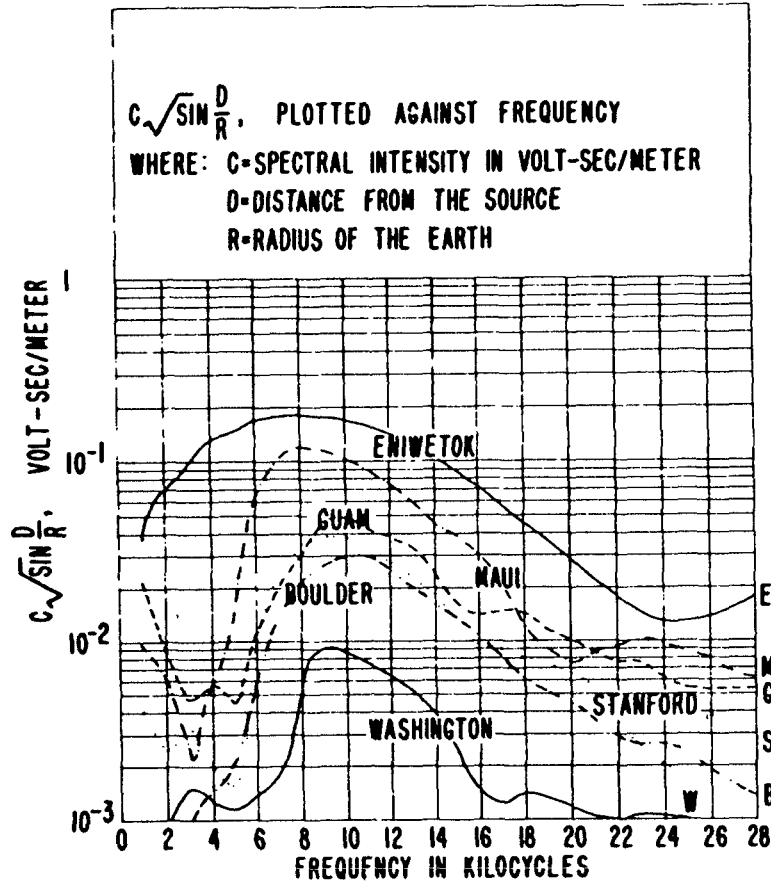
Figure 14 Spectral intensity, as a function of frequency, for Shot 2 as received at selected NBS stations.
