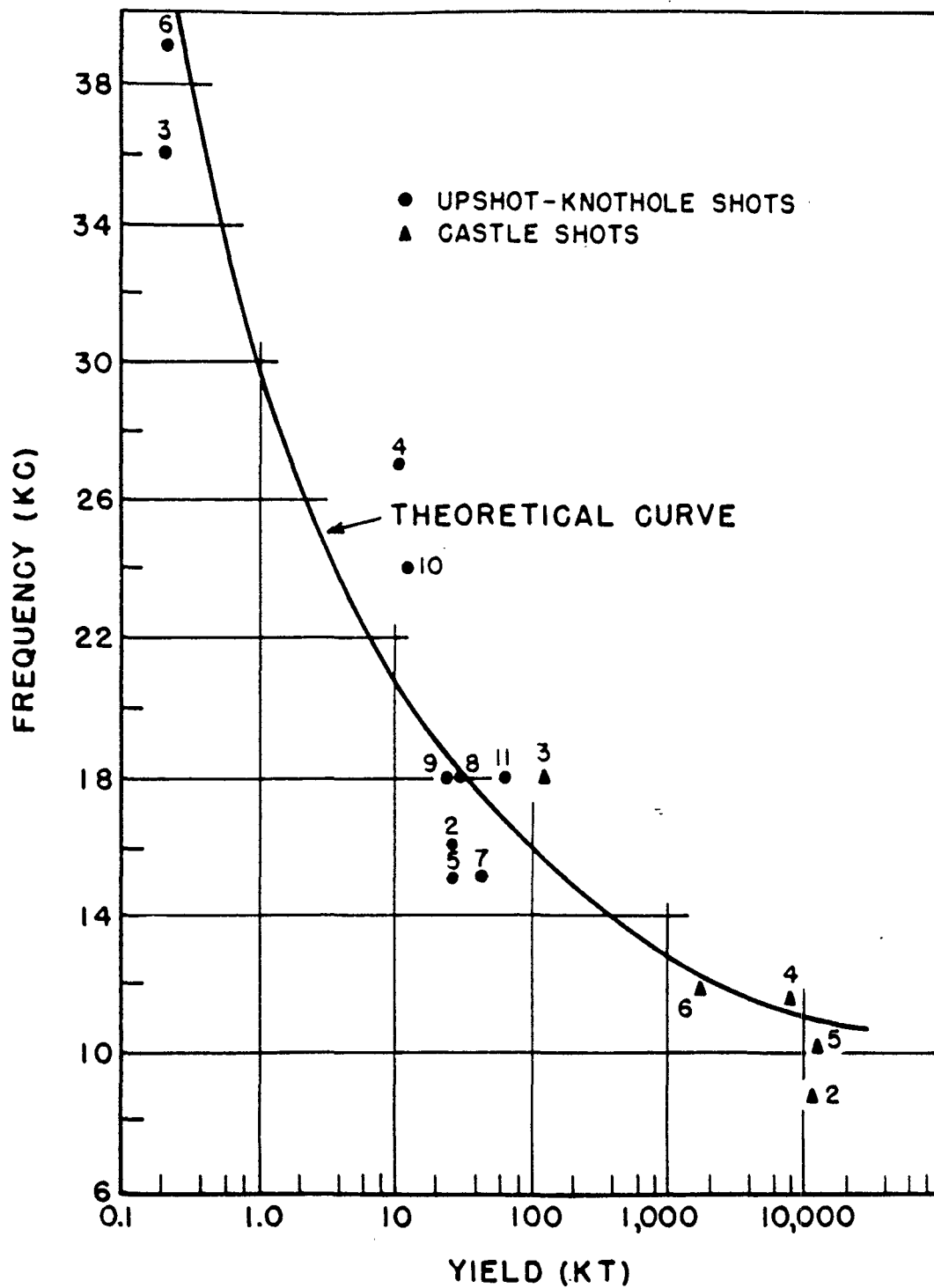
Figure 16 Plot of selected Upshot-Knothole and Castle close-in waveforms showing the relationship between yield and predominant frequency.
