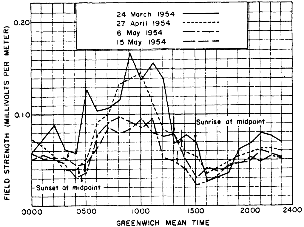
Figure 19 Plot of the field strength of NPM as measured by DRL at Thule, Greenland.
