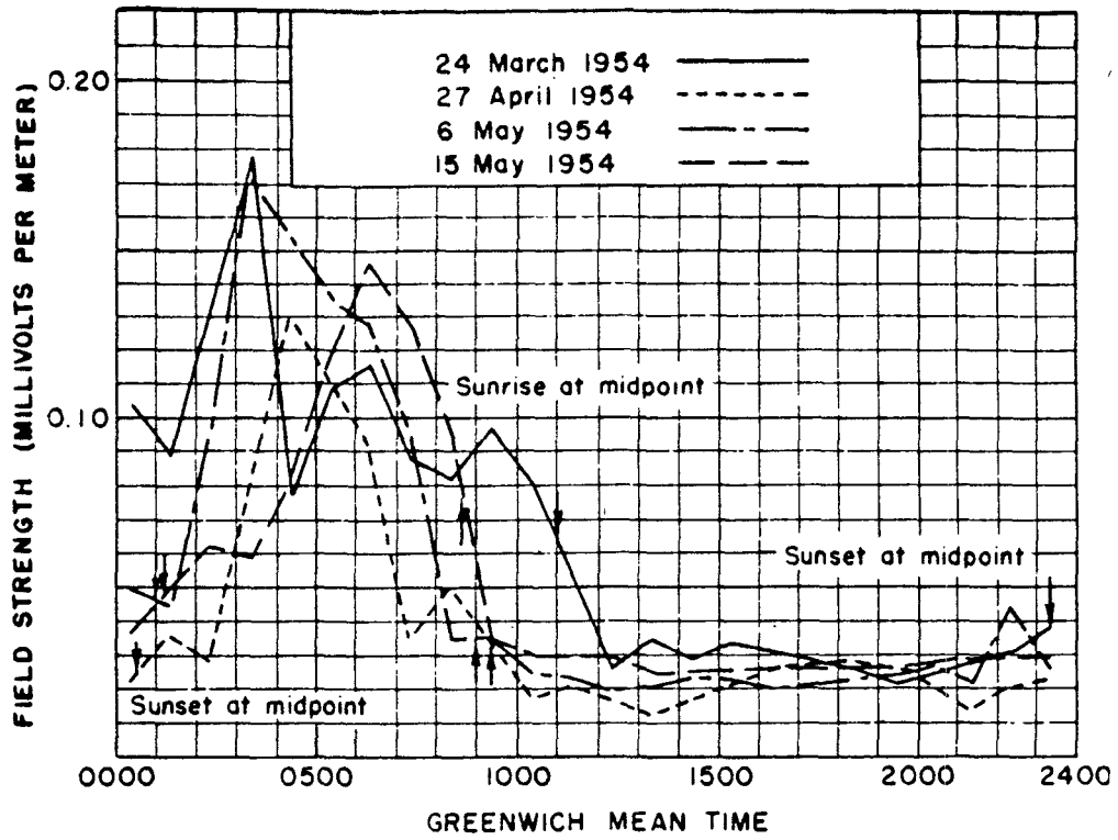
Figure 18 Plot of the field strength of NSS as measured by DRL at Thule, Greenland.
