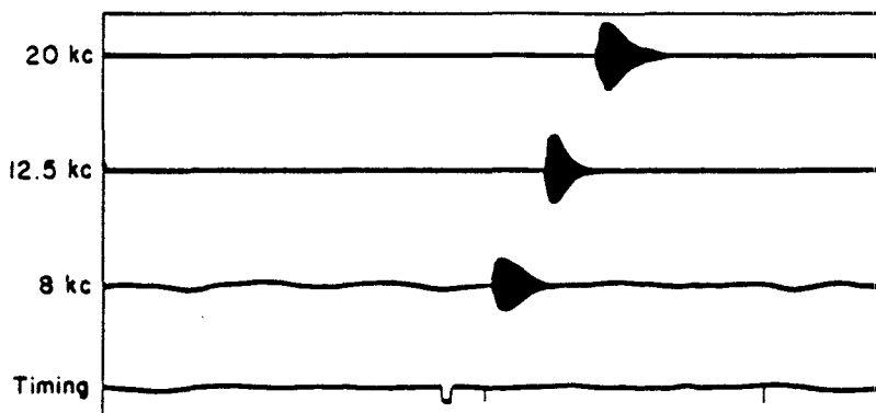
Figure 2 Typical NBS narrow-band field strength traces, with a timing trace recorded on a multi-beam oscilloscope at a distant location.
