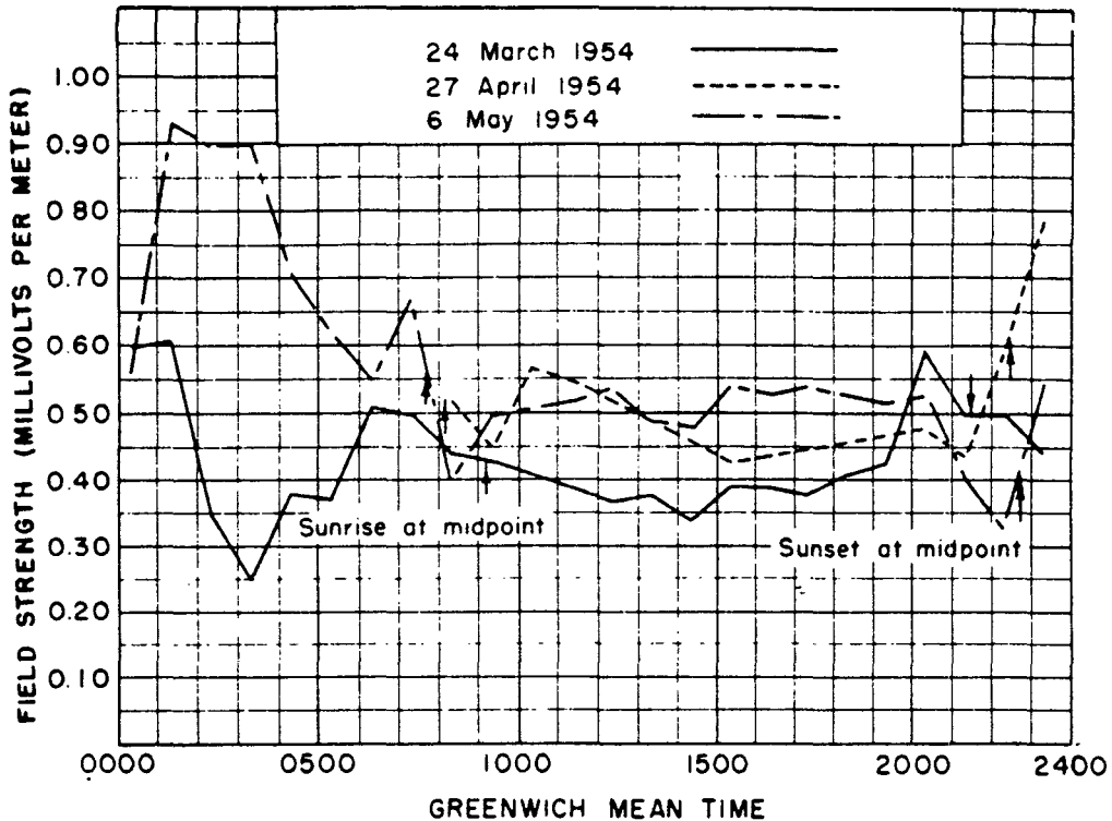
Figure 17 Plot of the field strength of NSS as measured by DRL at Kirknewton, Scotland.
