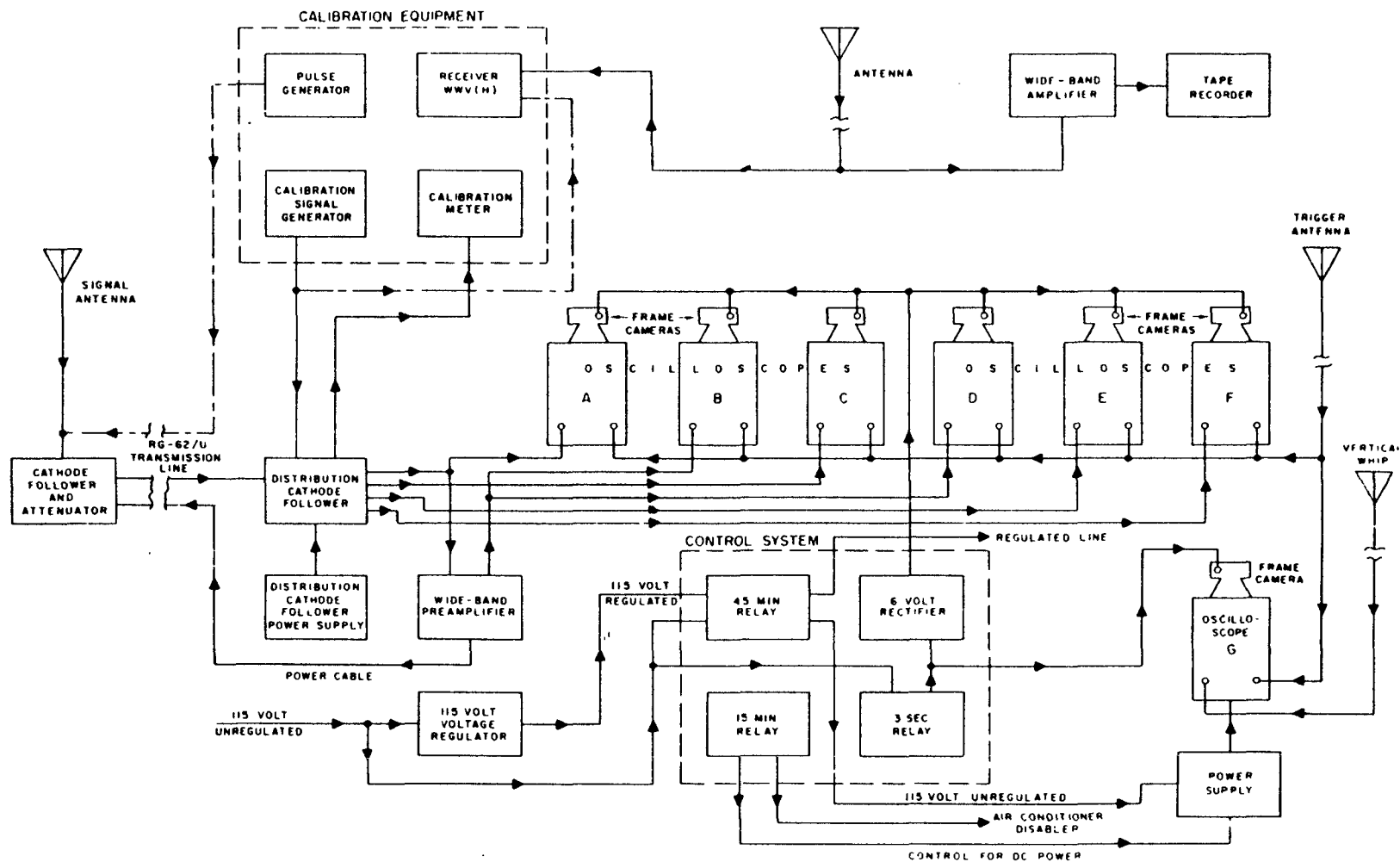
Figure 3 Block diagram showing the NBS close-in waveform instrumentation.
